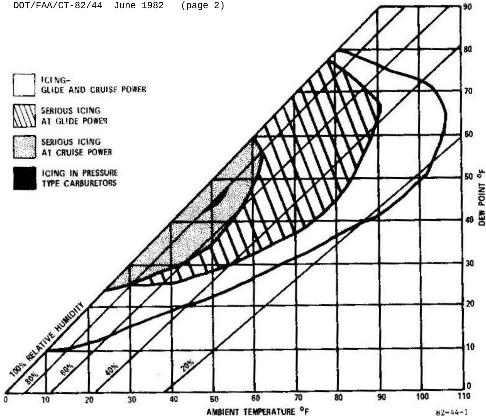
FIGURE 1. CARBURETOR ICING PROBABILITY CHART
