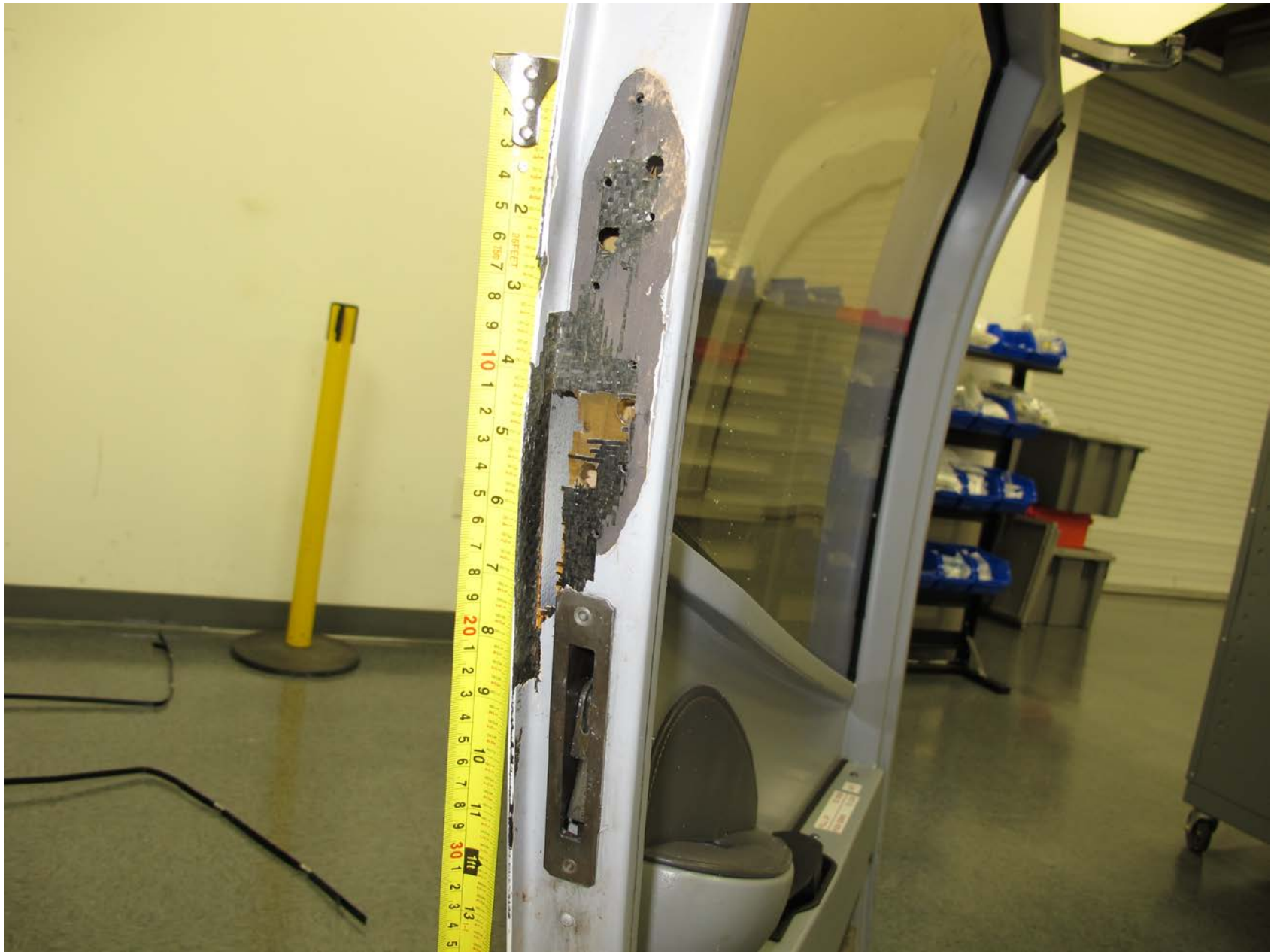
Photo 6 – View of door showing the missing door stop
