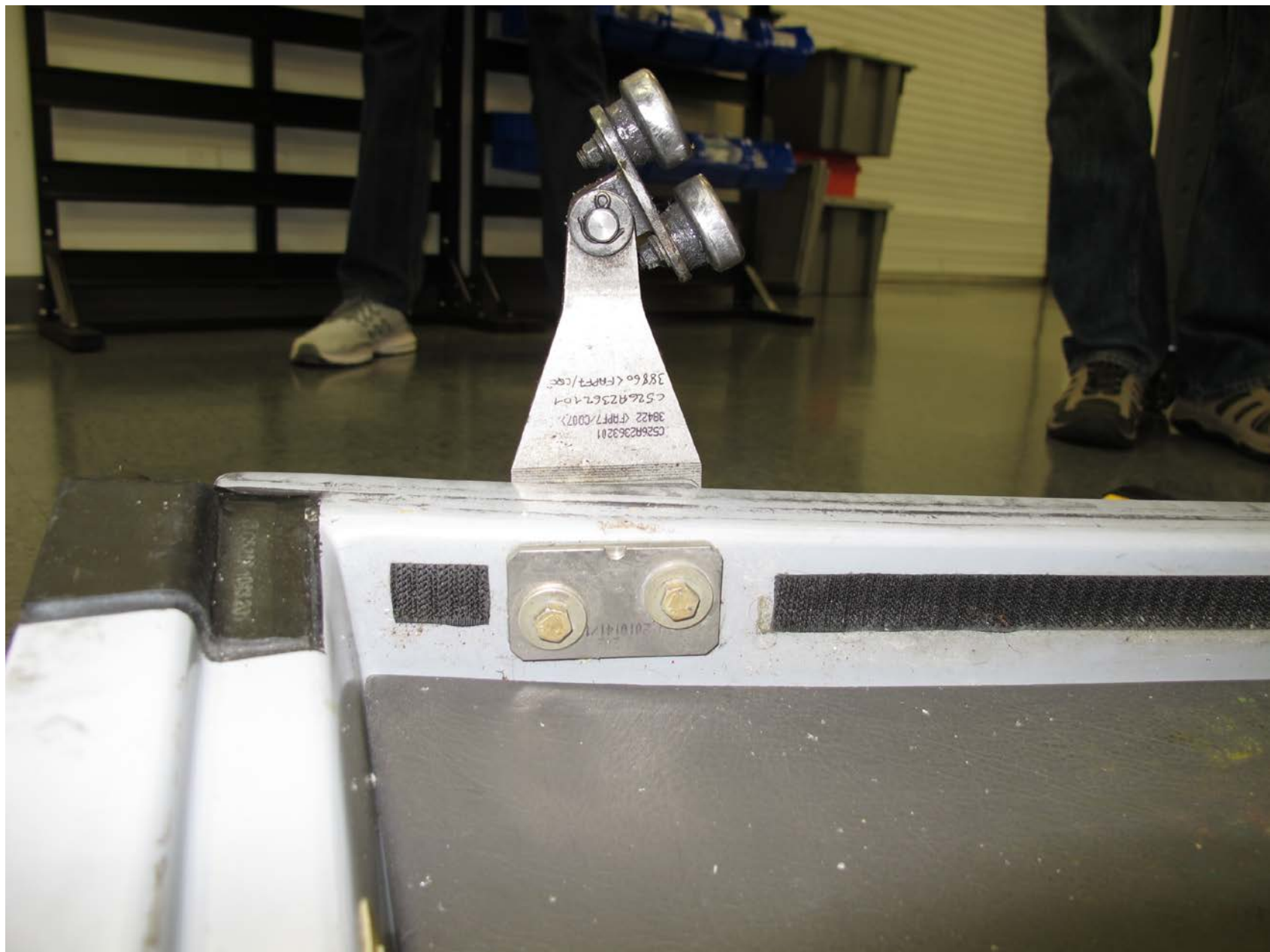
Photo 7 – View of door rail arm
