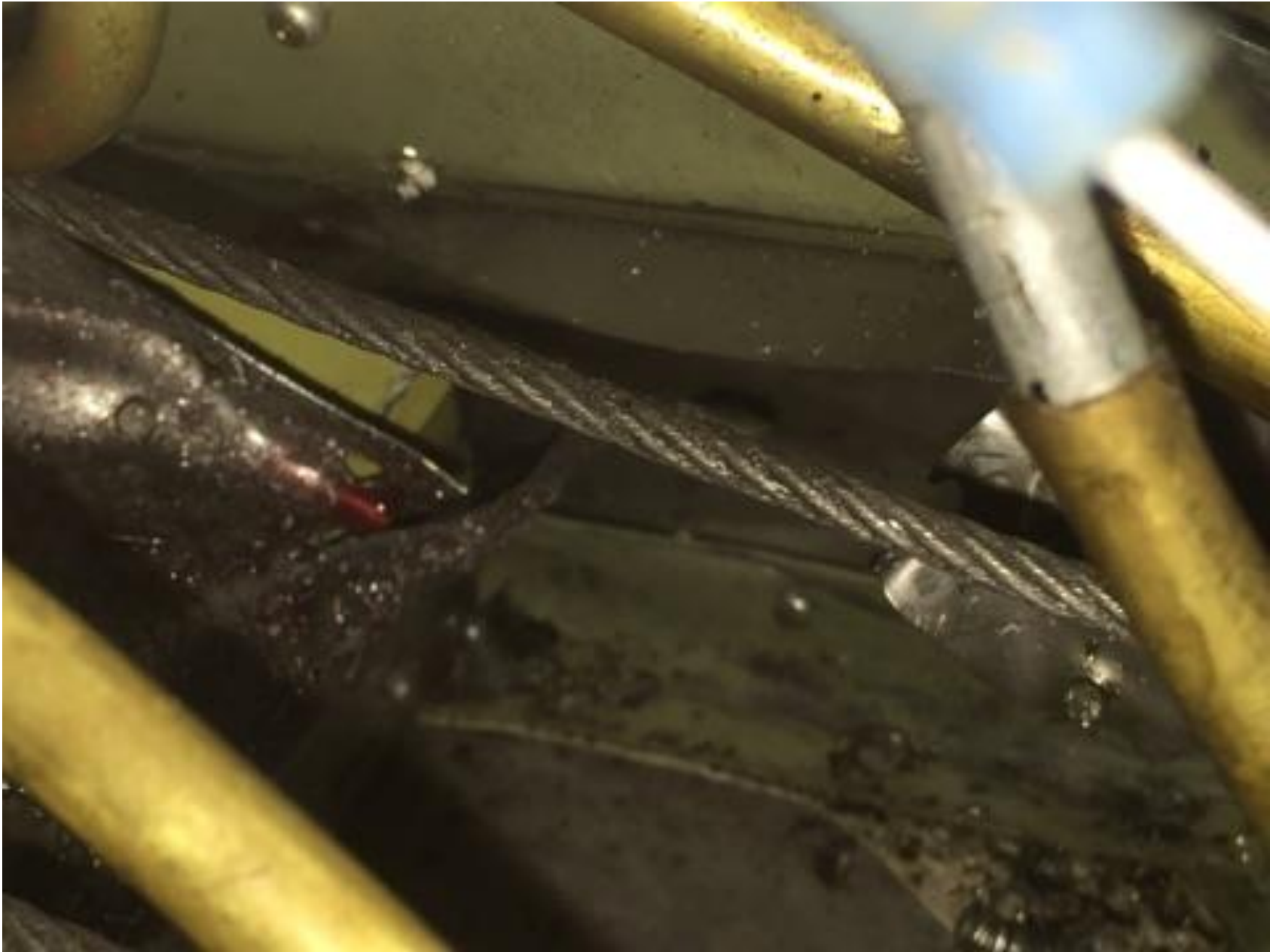
Photo 2 – Structural Damage (FAA Photo)
