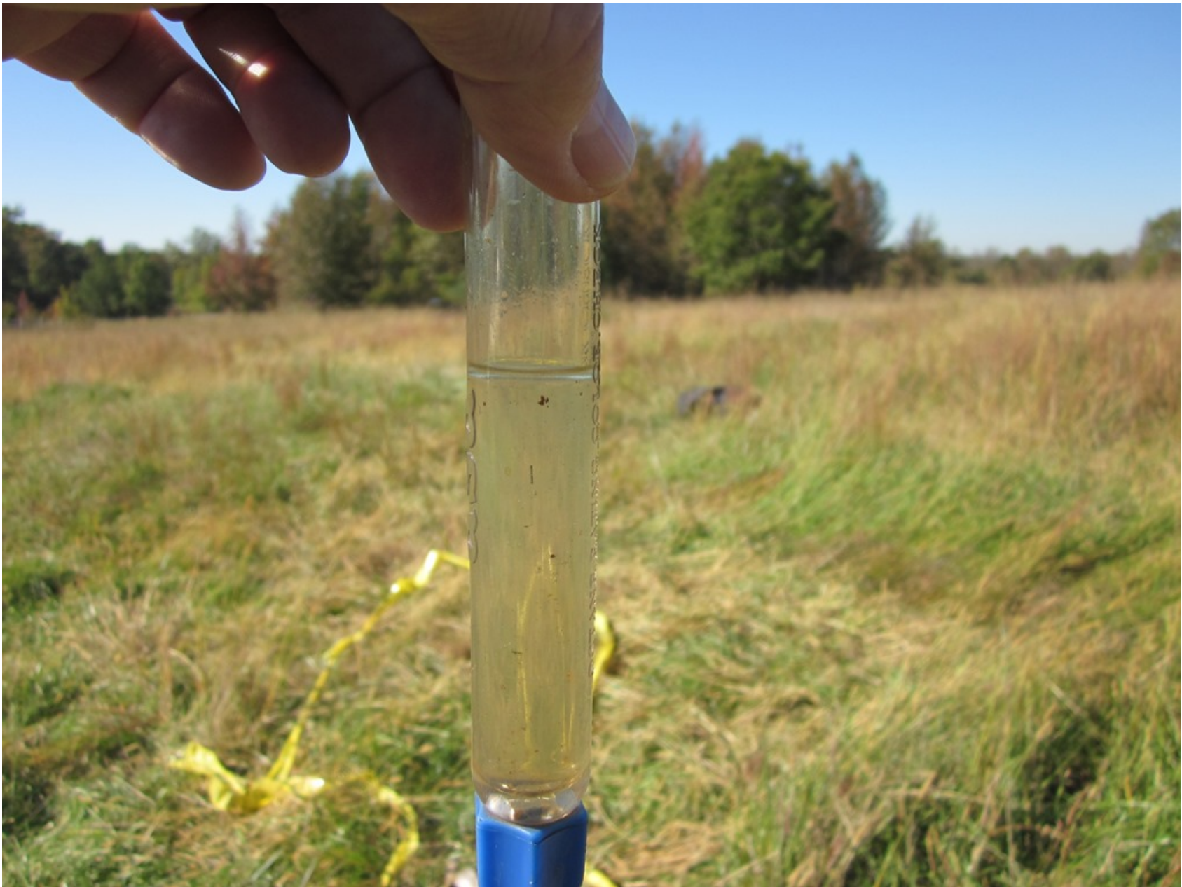
Photo 5 – Water Drained from Right Fuel Tank (FAA Photo)
