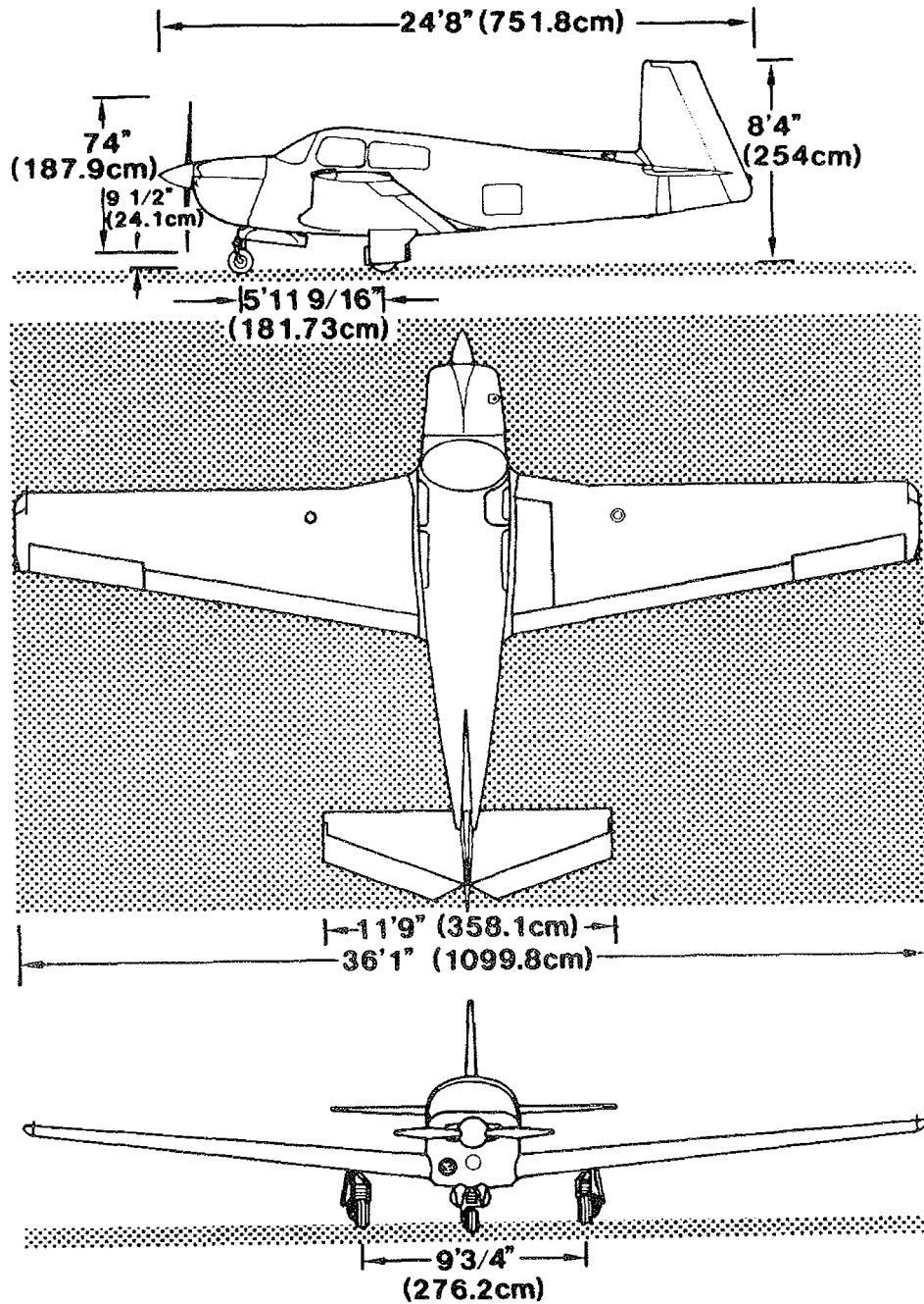
FIGURE 1-1 THREE VIEW
