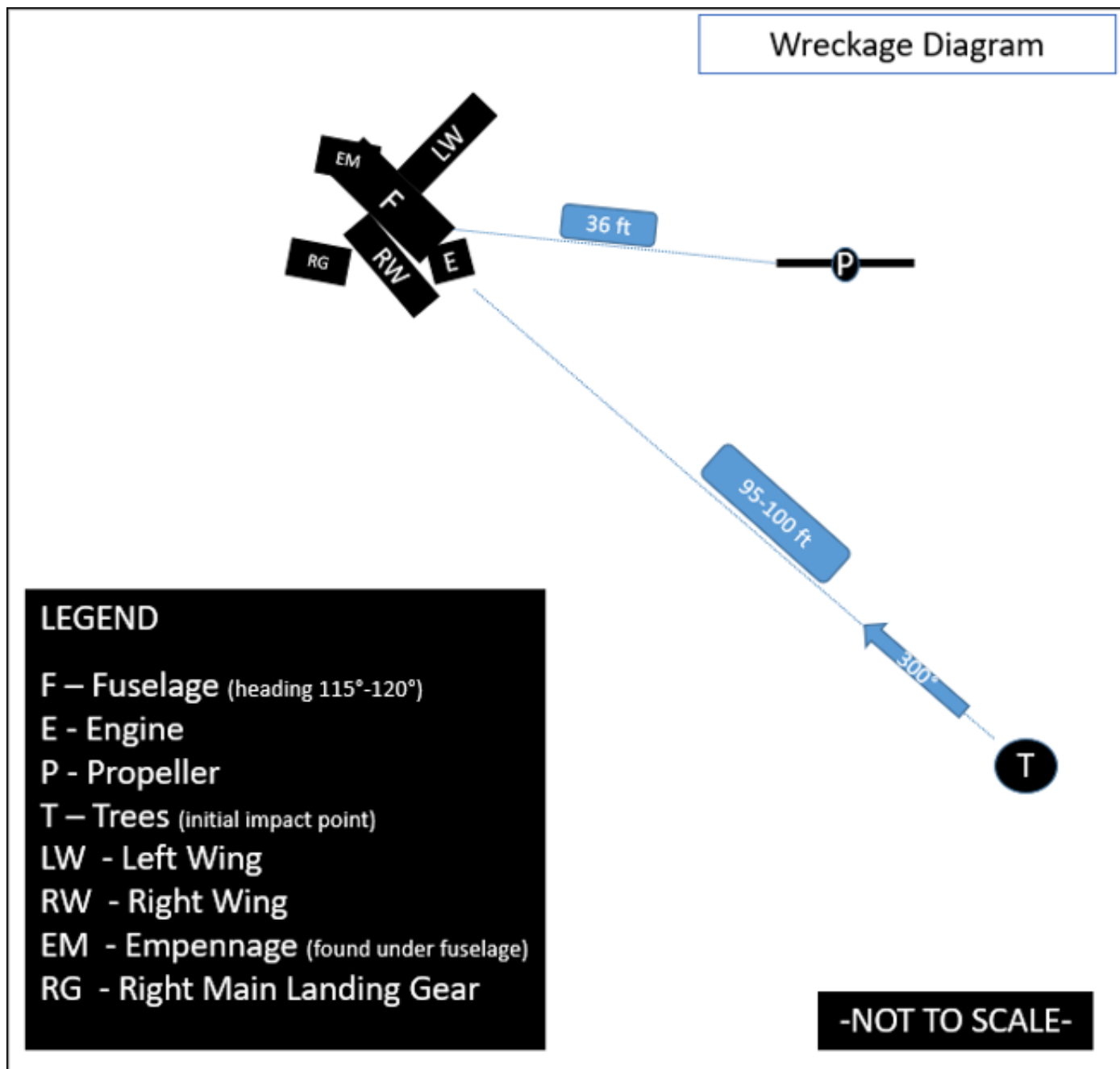
Photo 6 – Wreckage Diagram
