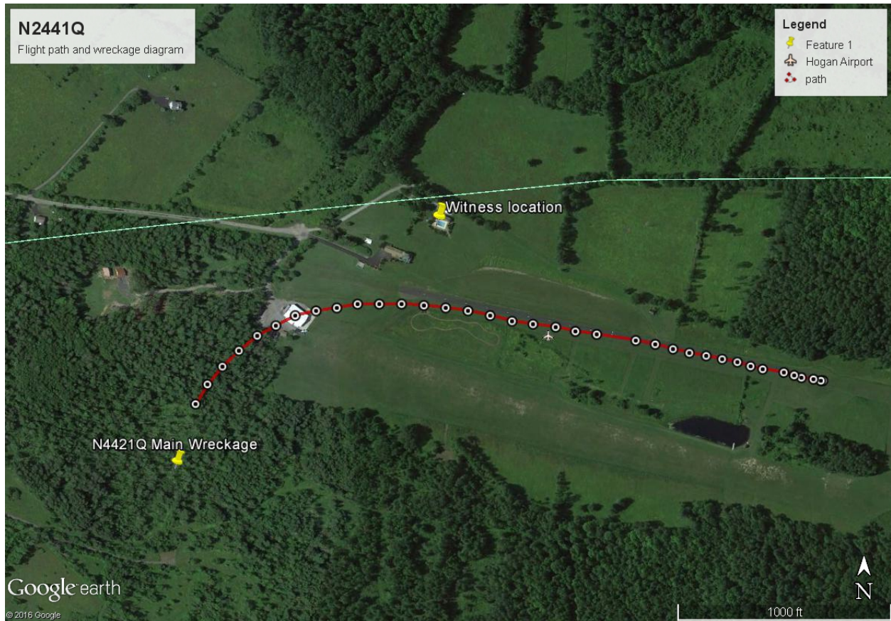
Figure 1 Wreckage diagram with flight track data overlaid on a Google Earth image.
