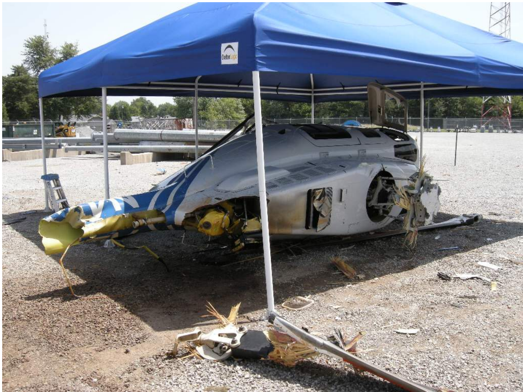
Photo 1 – Main Wreckage, View of Top of Fuselage (NTSB Photo)
