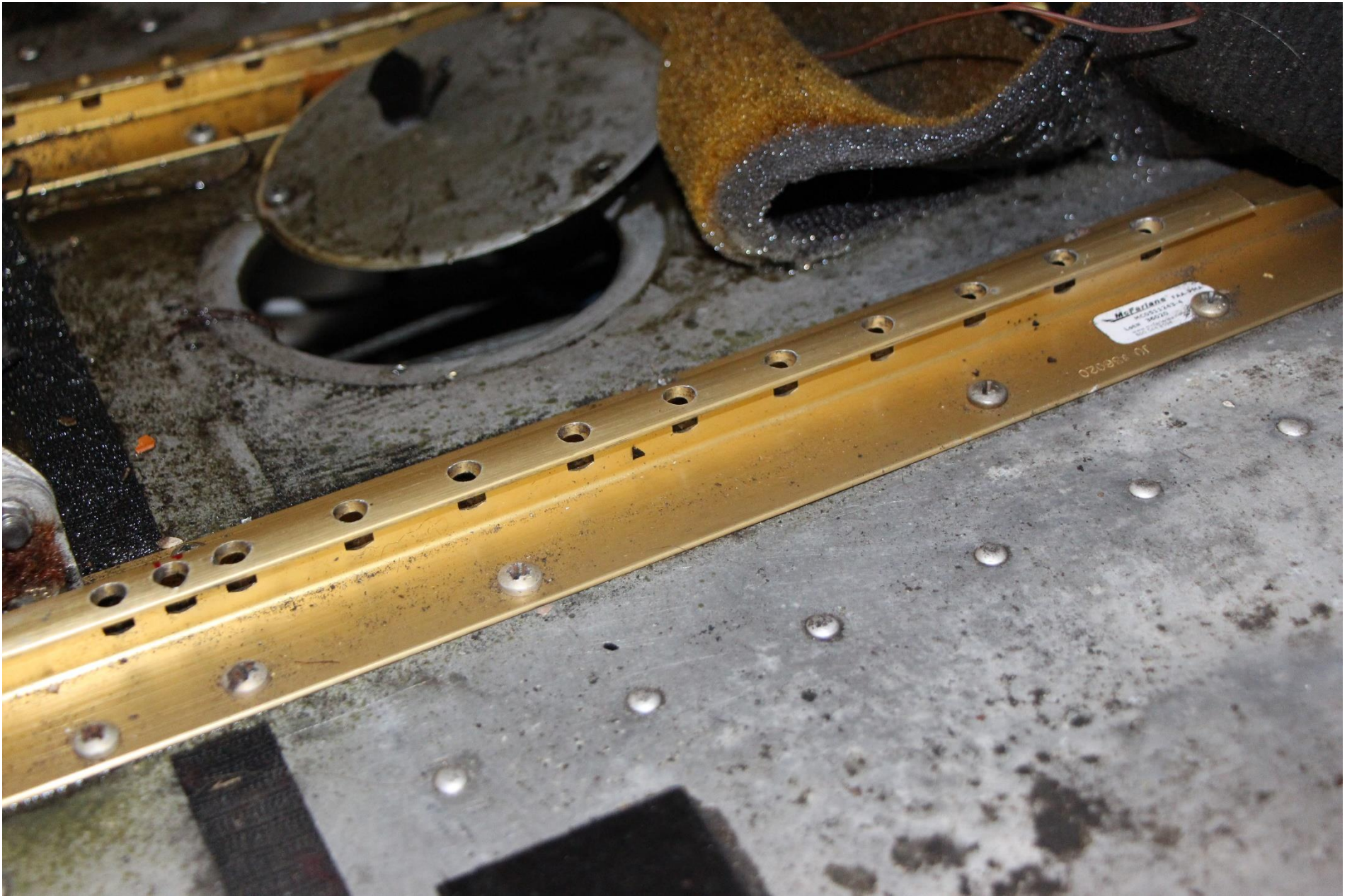
Photo 5 – seat rail impression marks on 11th hole – (Textron)
