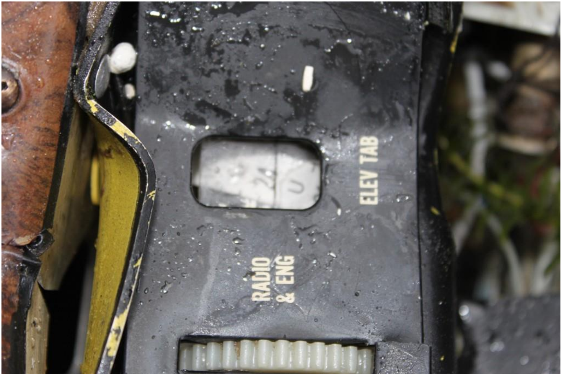
Photo 10 - NTSB Digital Photograph. View of the Elevator Trim Indicator
