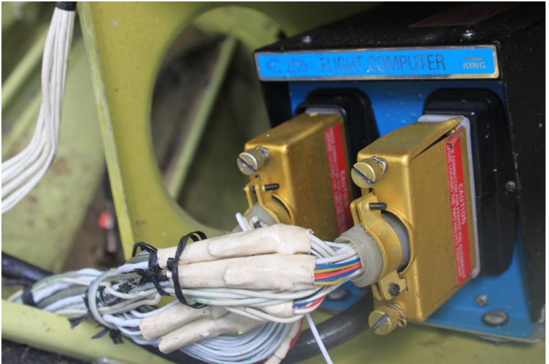
Photo 13 - NTSB Digital Photograph. View of the Connections at the Autopilot Flight Computer
