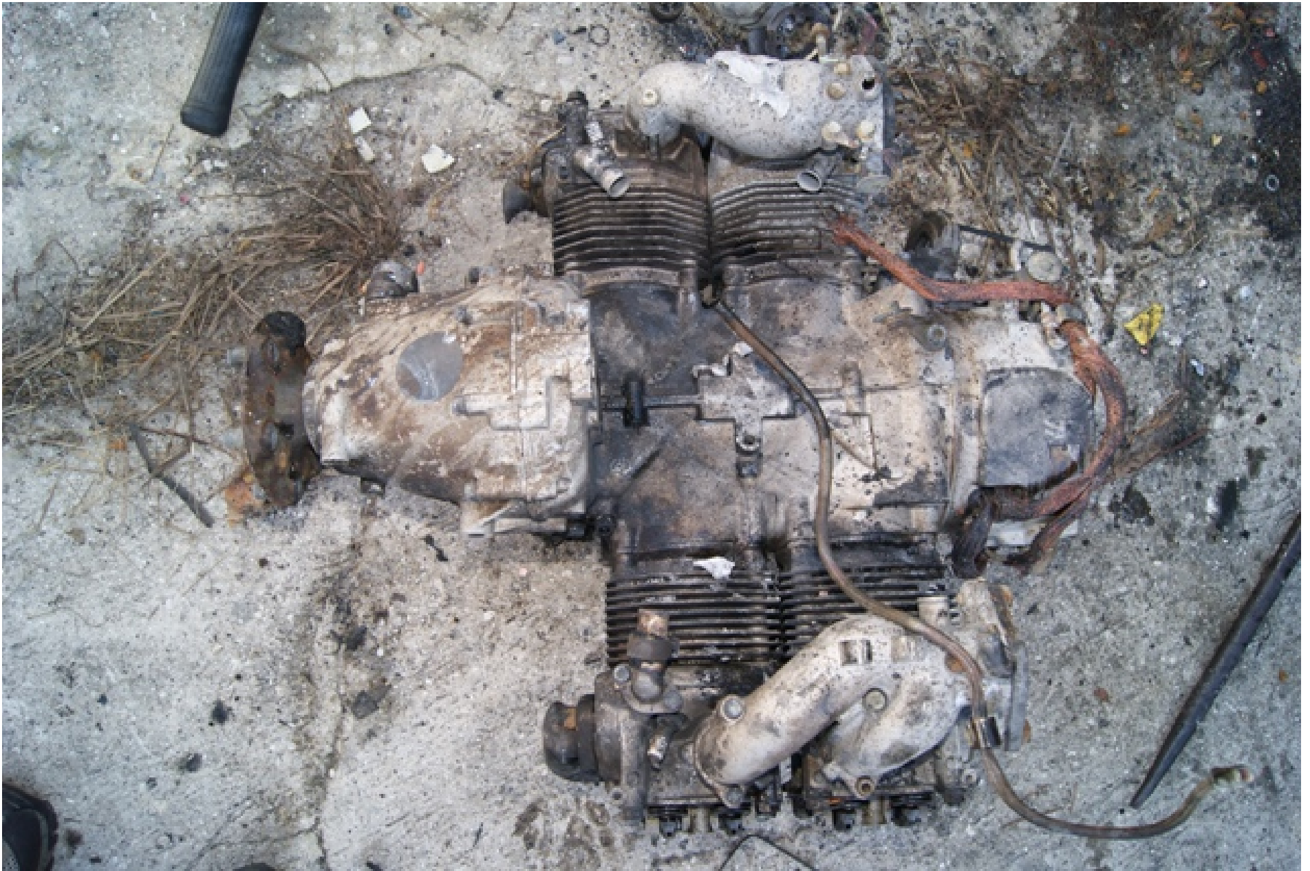
Photo 13 – Top View of Engine
