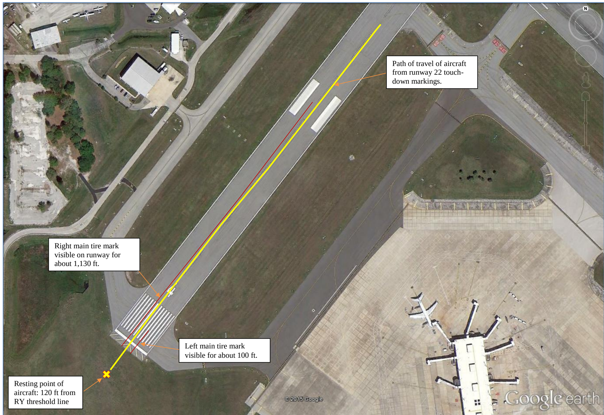
Figure 1 Illustrated airport diagram
