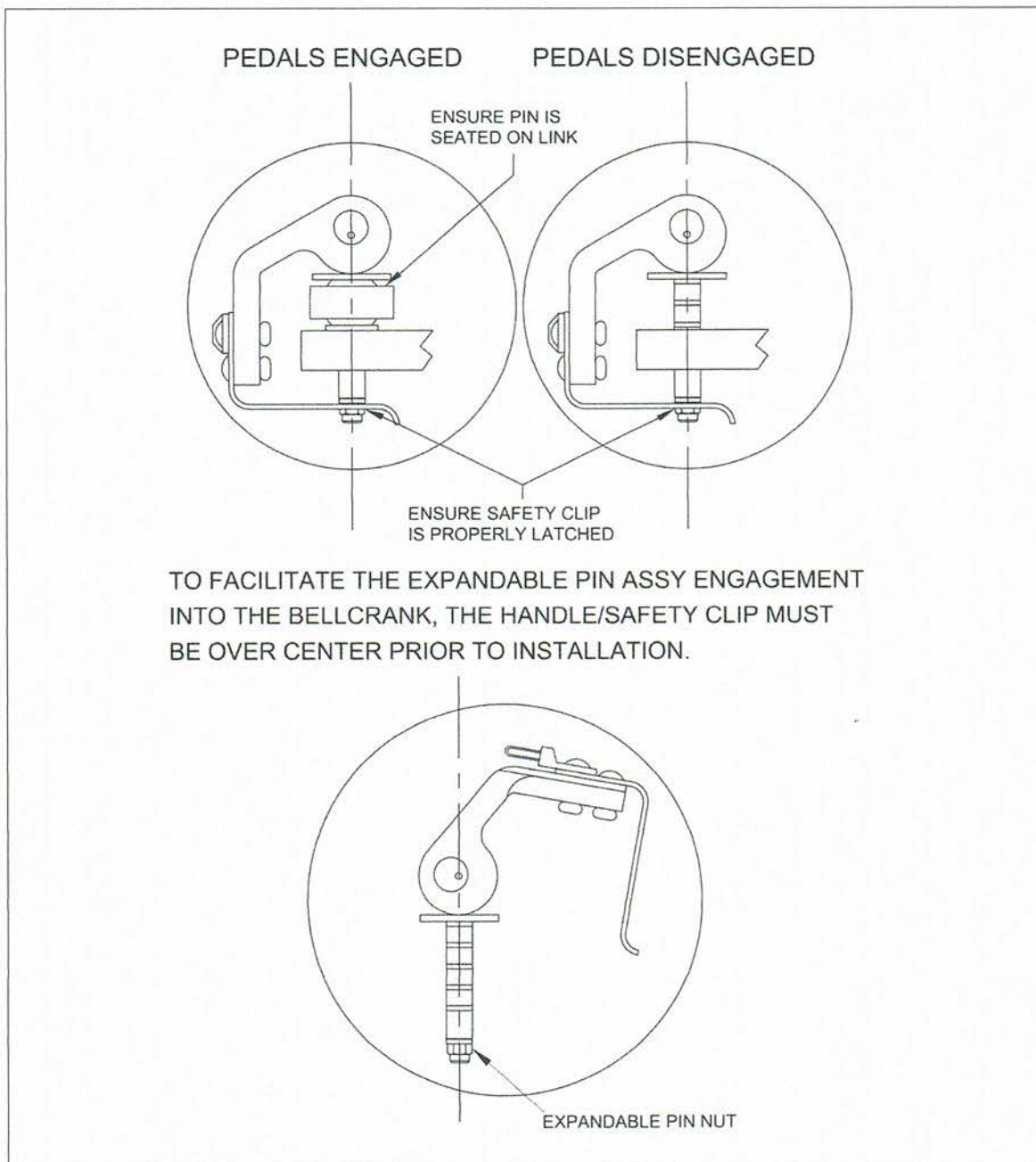
FIGURE 2. EXPANDABLE PIN ASSEMBLY ENGAGEMENT
