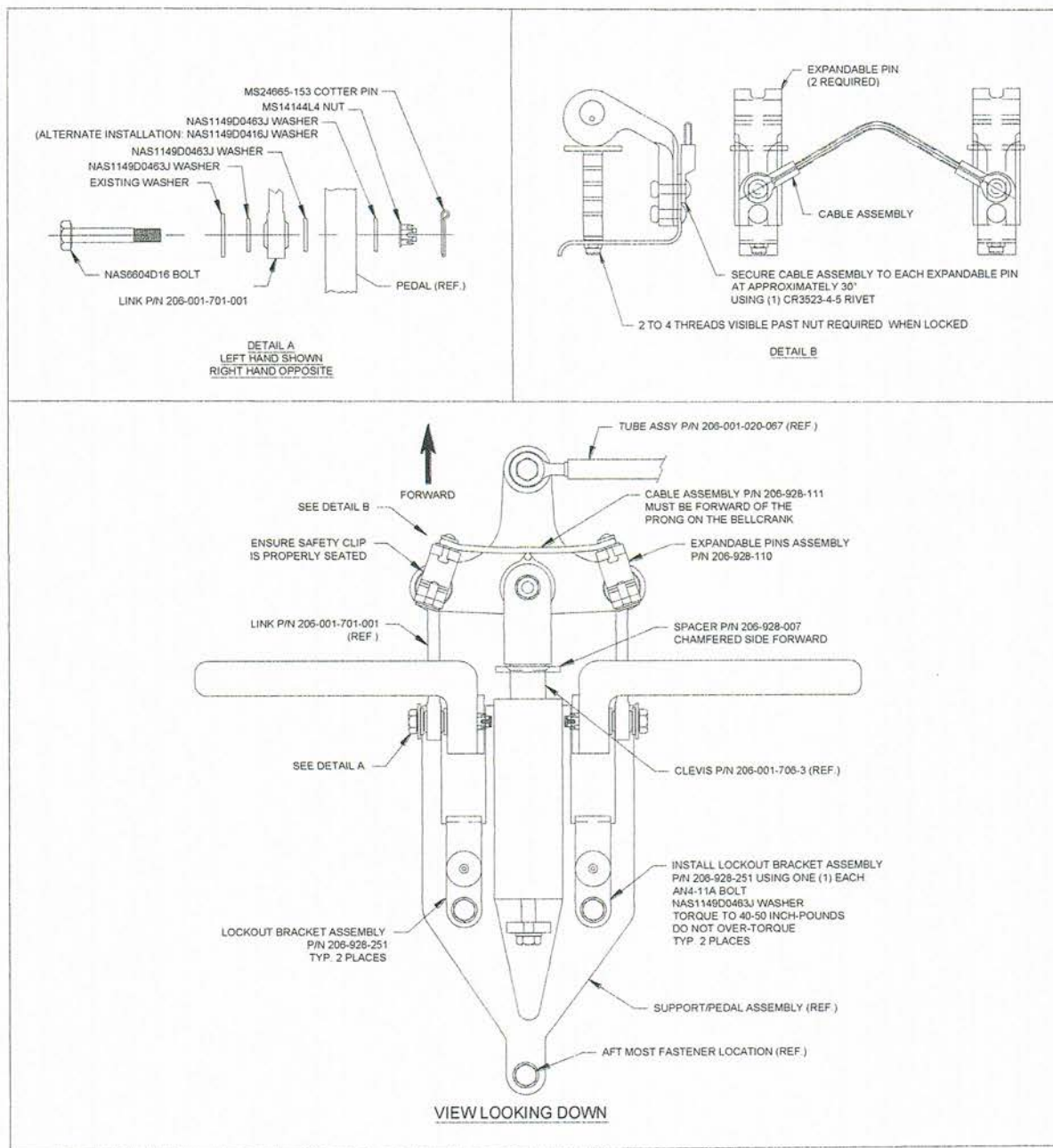
FIGURE 1. TAIL ROTOR PEDAL LOCKOUT KIT INSTALLATION
