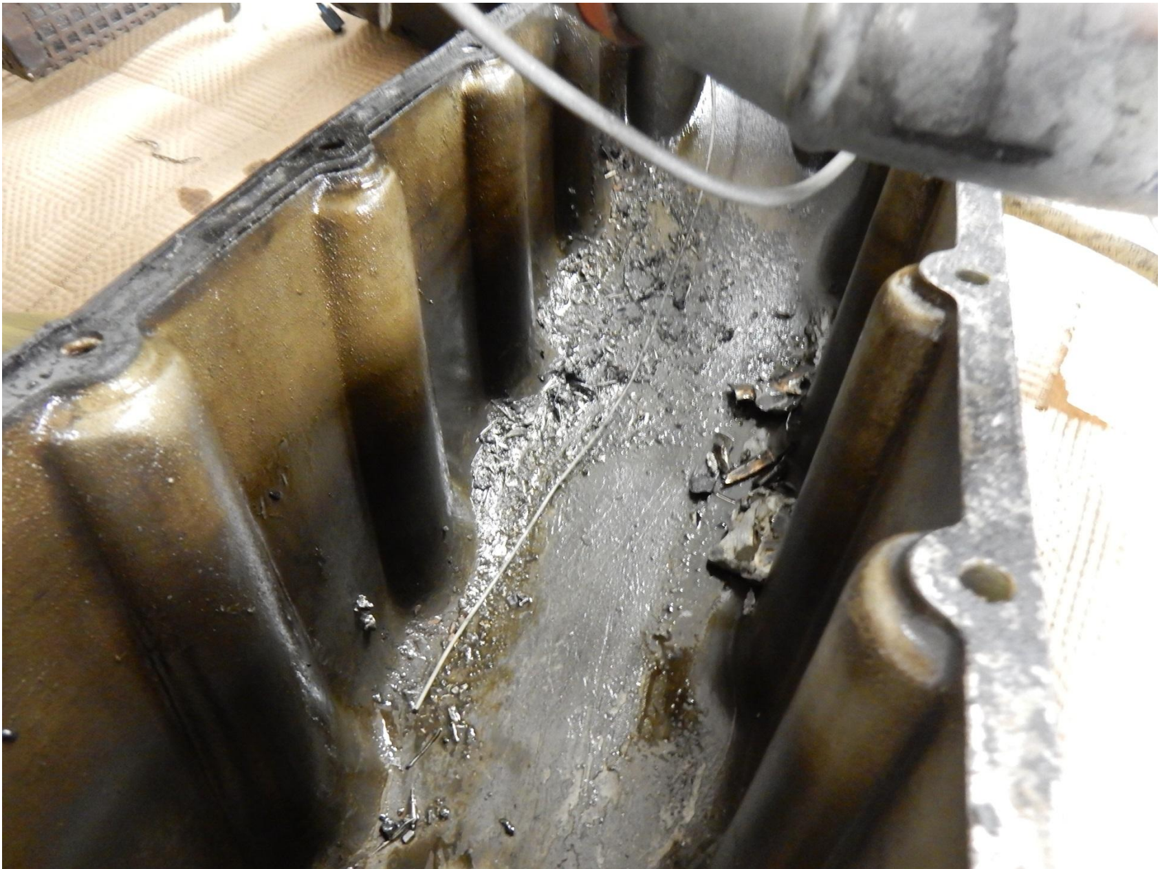
Photo 5 – View of Metal Fragments and Bearing Material in Oil Sump as Found (FAA)
