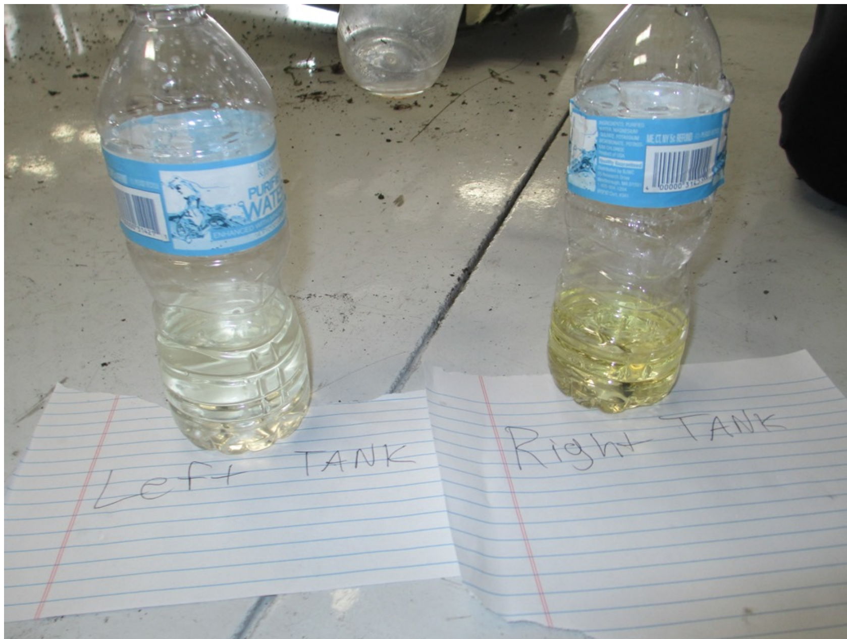
Photo 5 - Water Drained from LH and RH Fuel Tanks
