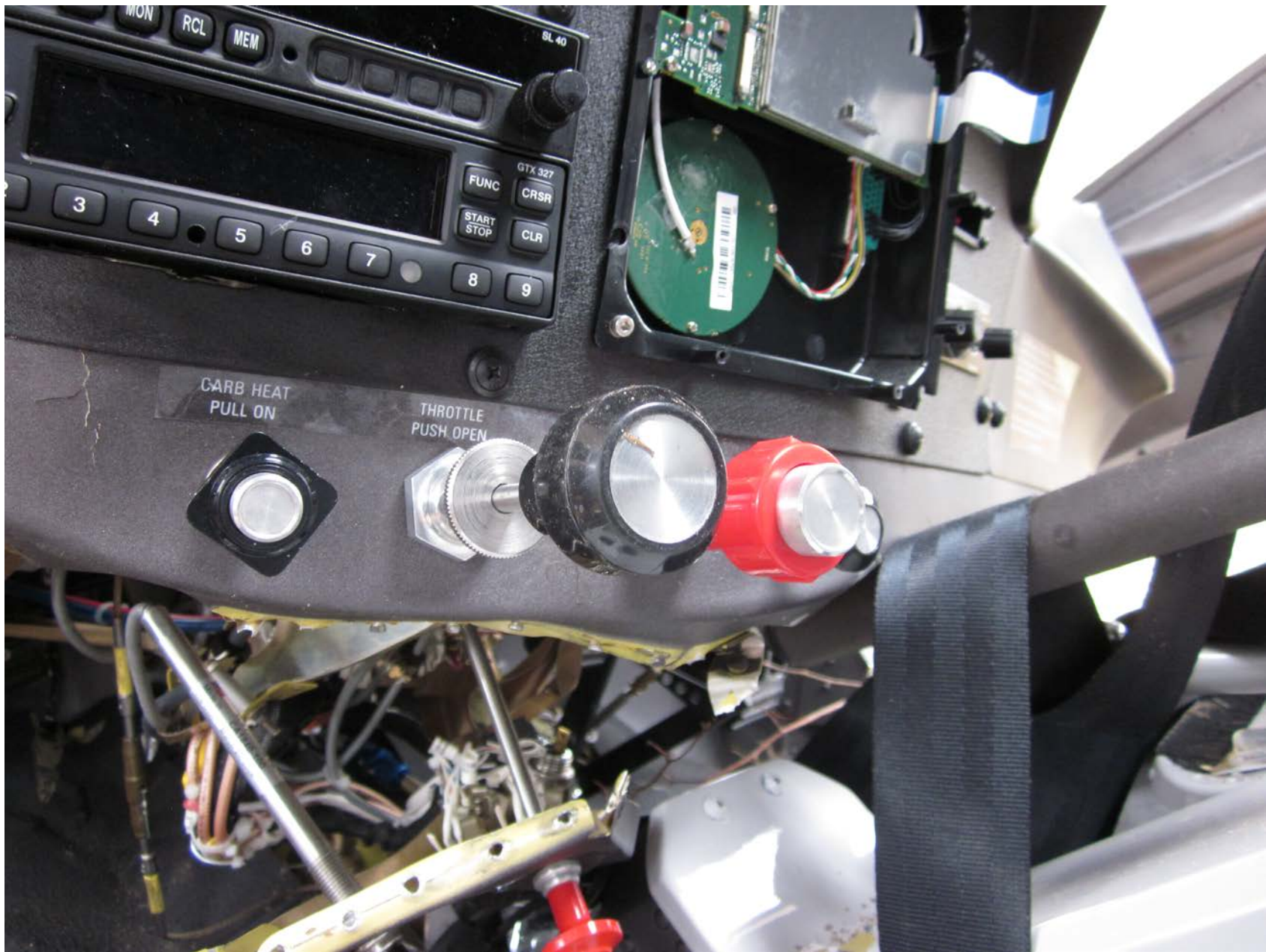
Photo 5 - Throttle and Mixture as Found (Courtesy of FAA)
