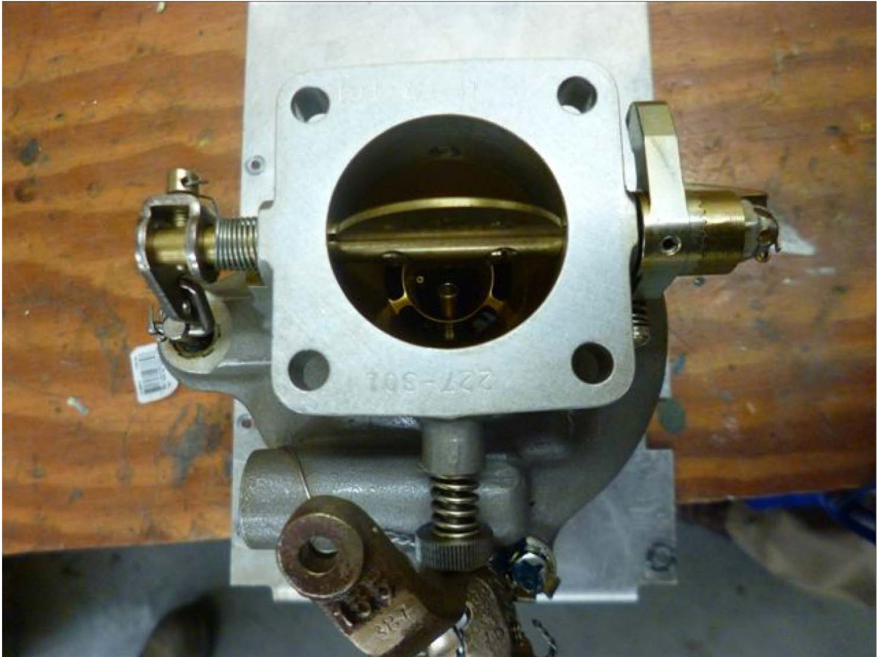
Photo 9 – Carburetor Throttle Valve – Courtesy of AIG Aerospace
