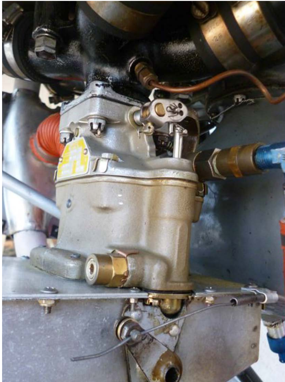
Photo 7 – Carburetor – Courtesy of AIG Aerospace
