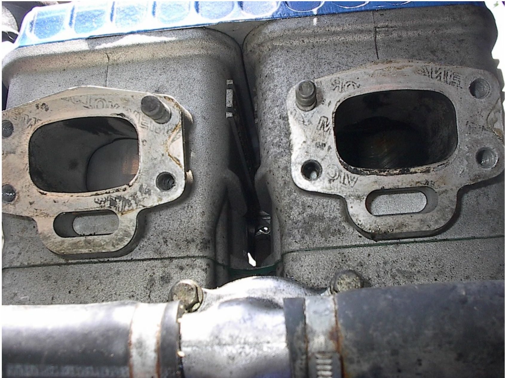
Photo 3 - Digital Photograph Provided by Owner. View Depicting the Piston Sides of the Forward Cylinder. No Scuffing or Scoring was Noted on the Piston. Hone marks are Visible on the Rear Cylinder Walls
