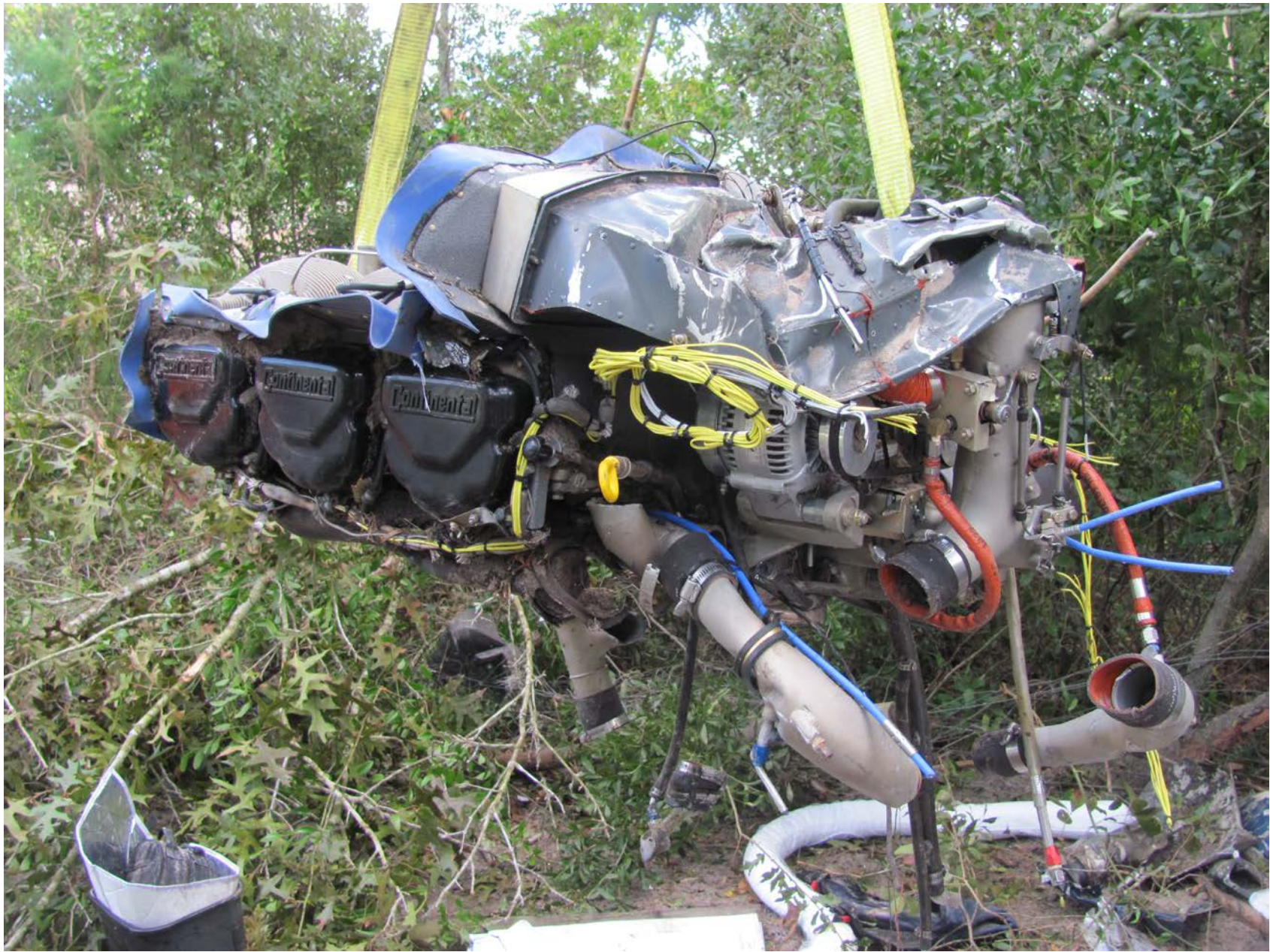
Photo 4 – Engine Left Side View
