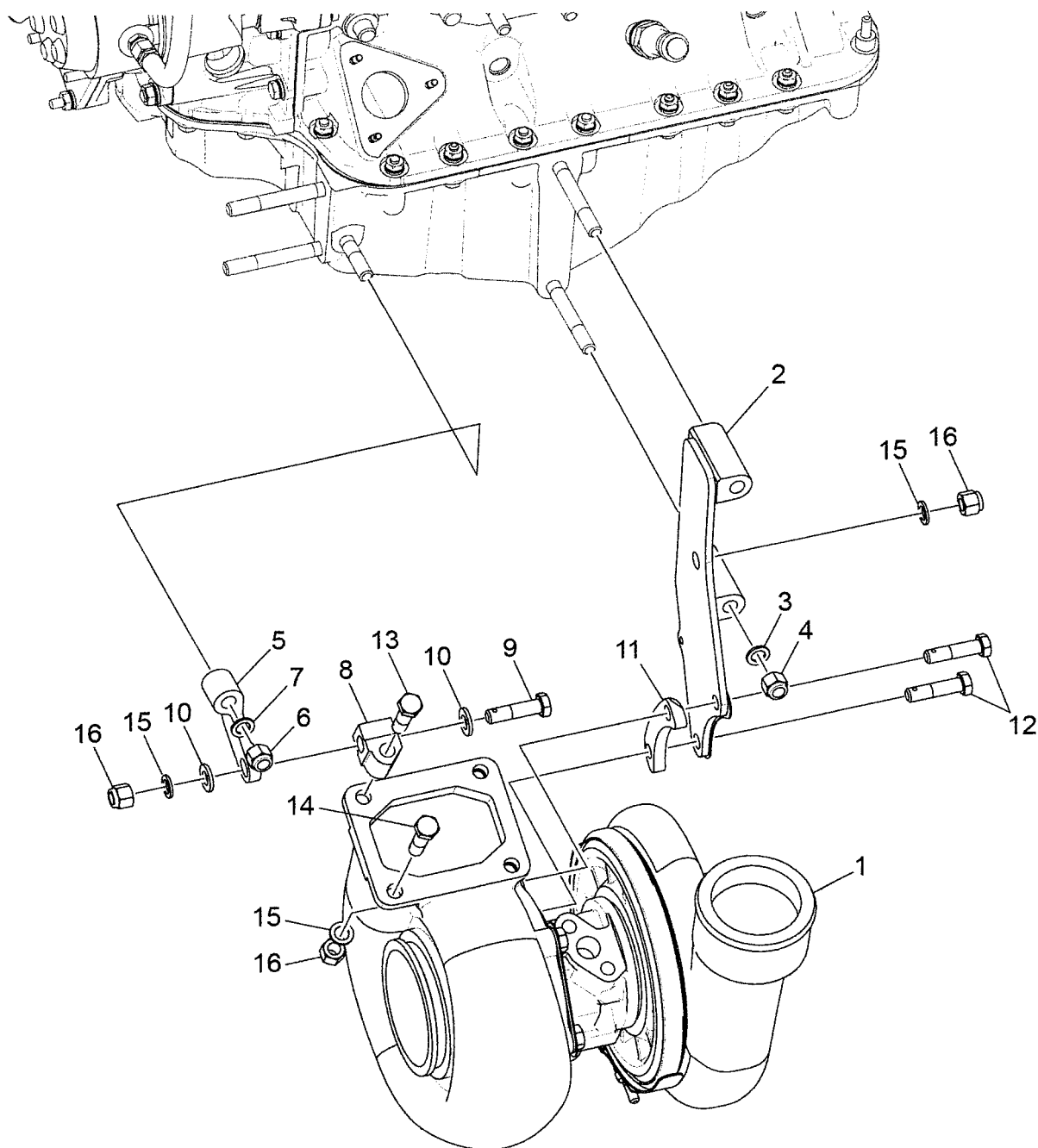
Figure 13 Turbocharger, Supports, and Attaching Parts
