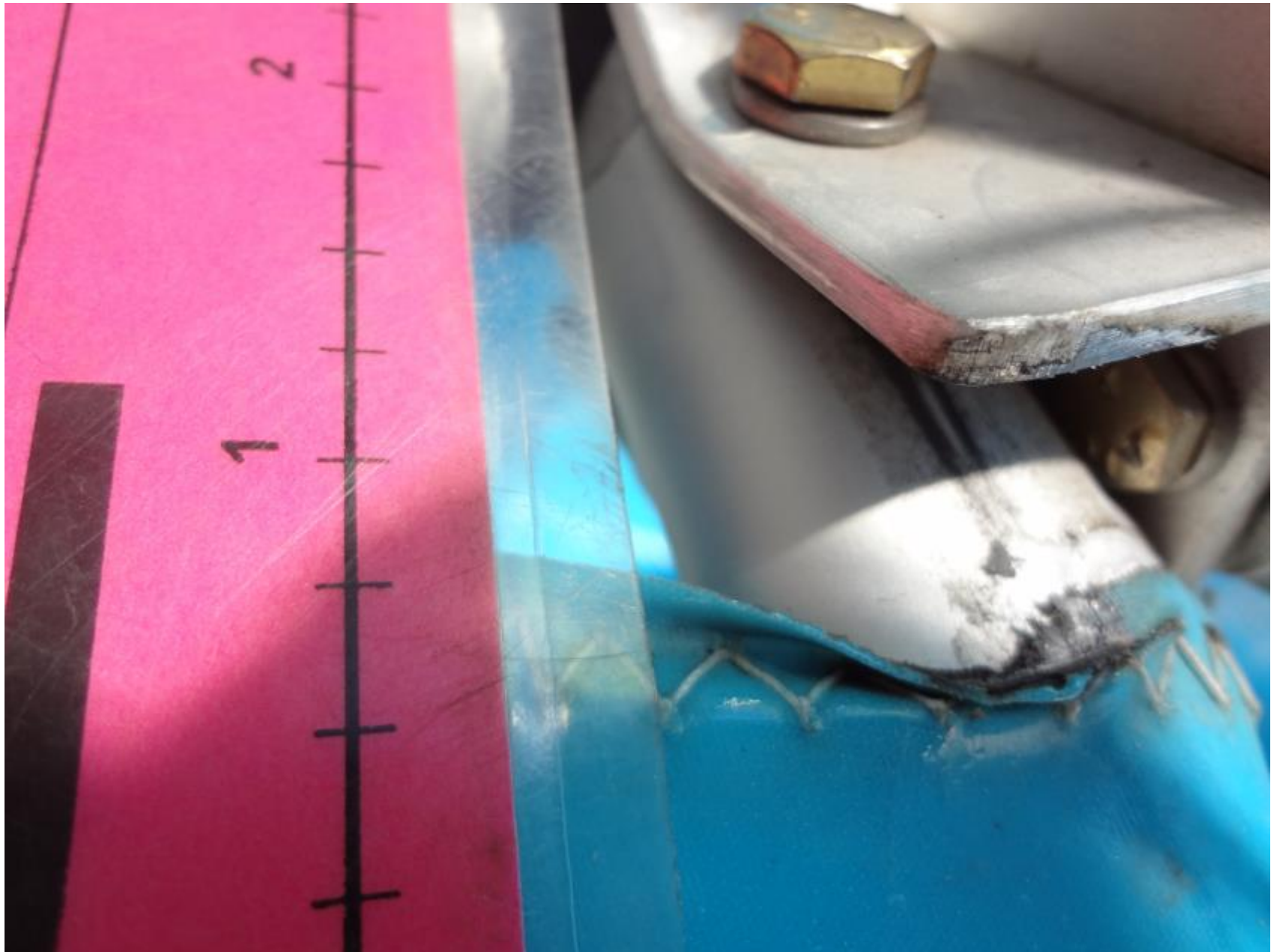
Photo 4 – Upper Channel Elevator Horn as Viewed
