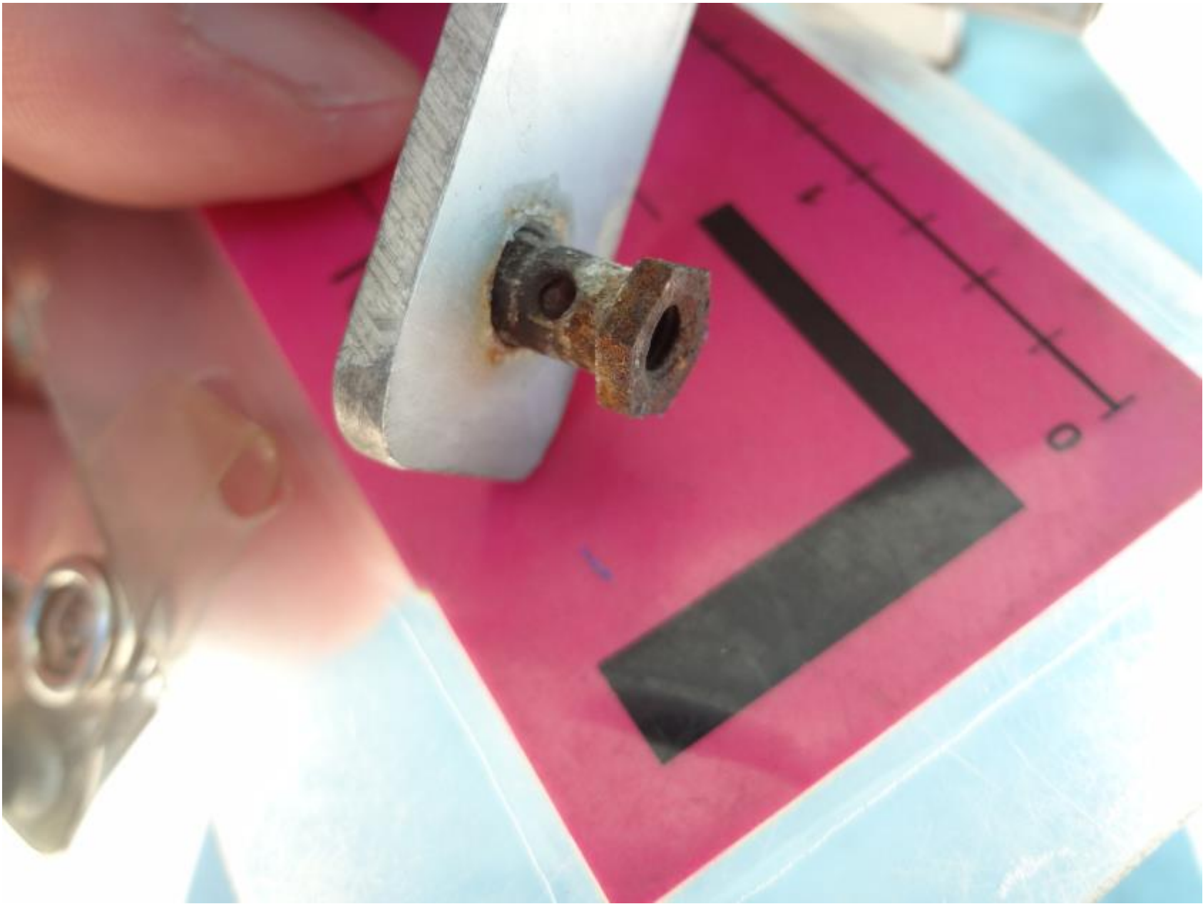
Photo 5 - Elevator Cable Clamp as Viewed
