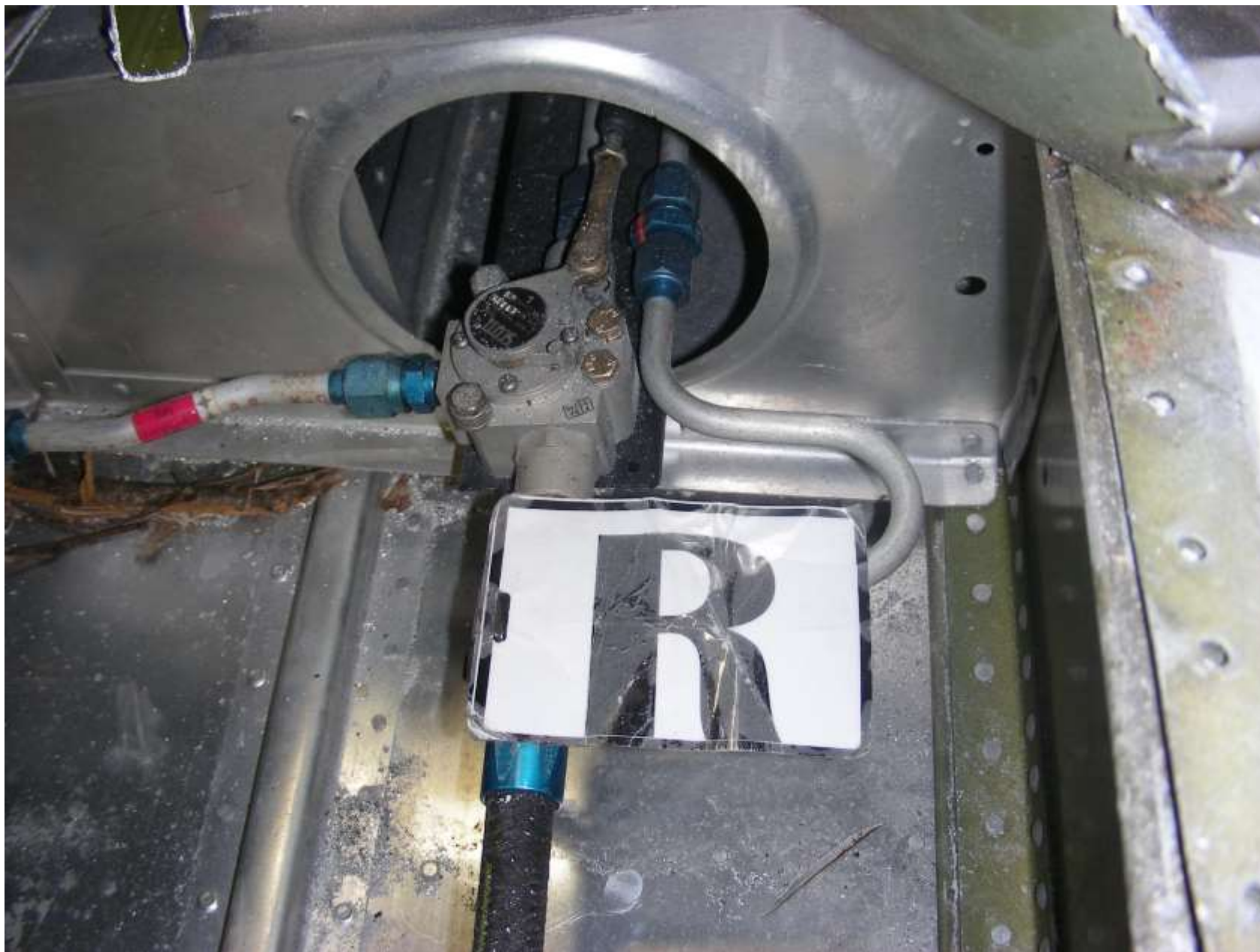
Photo 8 – Right Fuel Selector Valve
