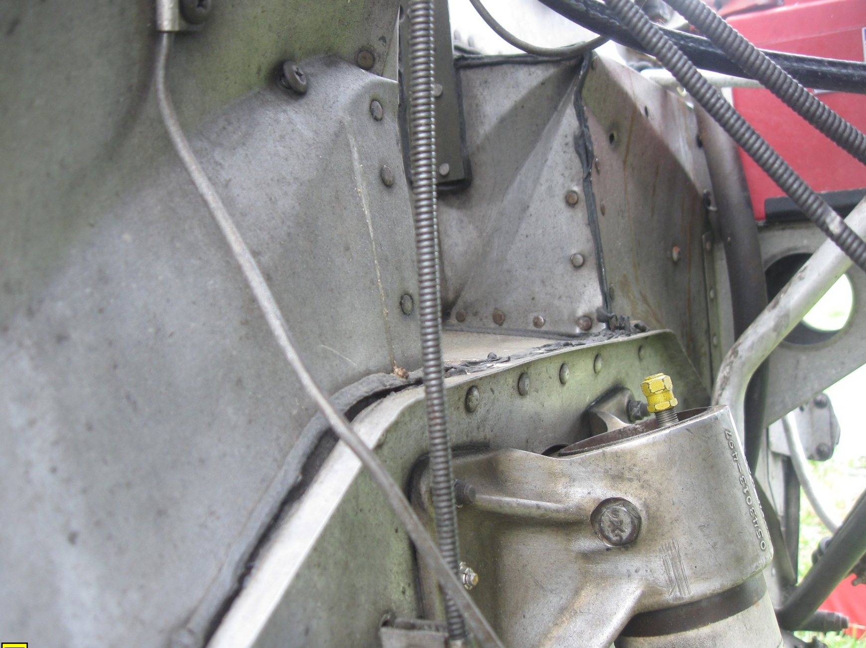
Photo 1 - Damaged Firewall
