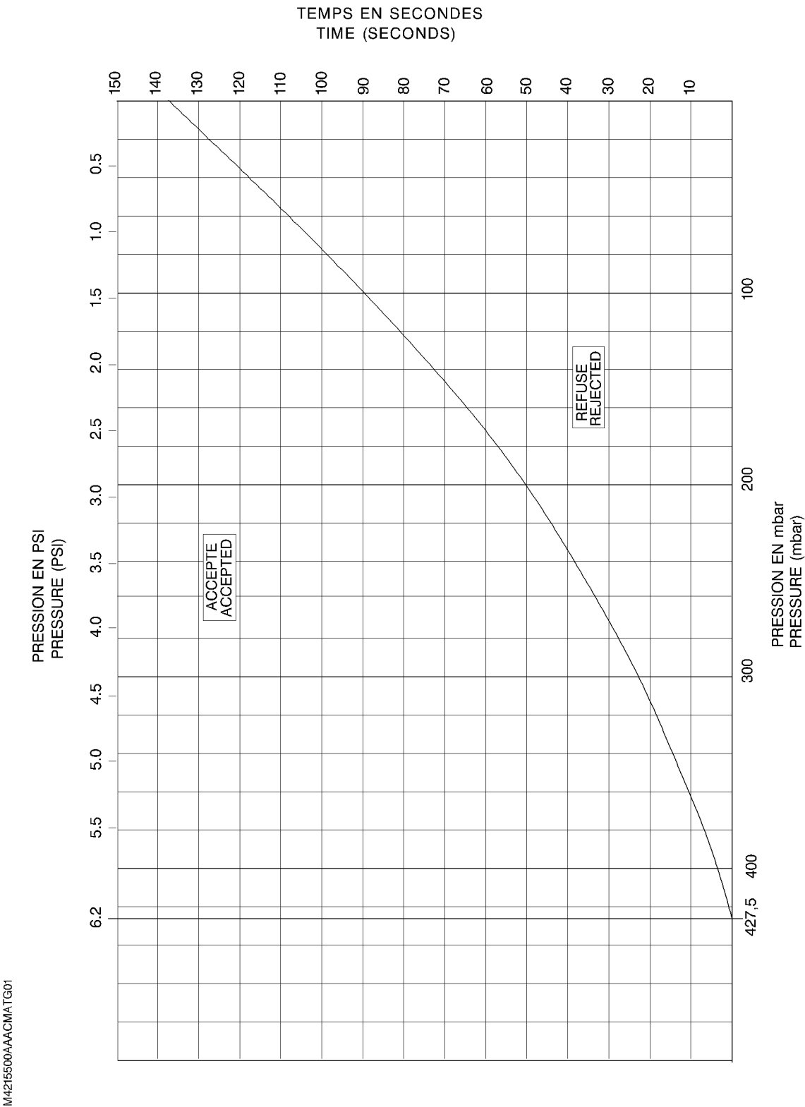
Cabin leak rate chart Table 501 - Without pilot door
