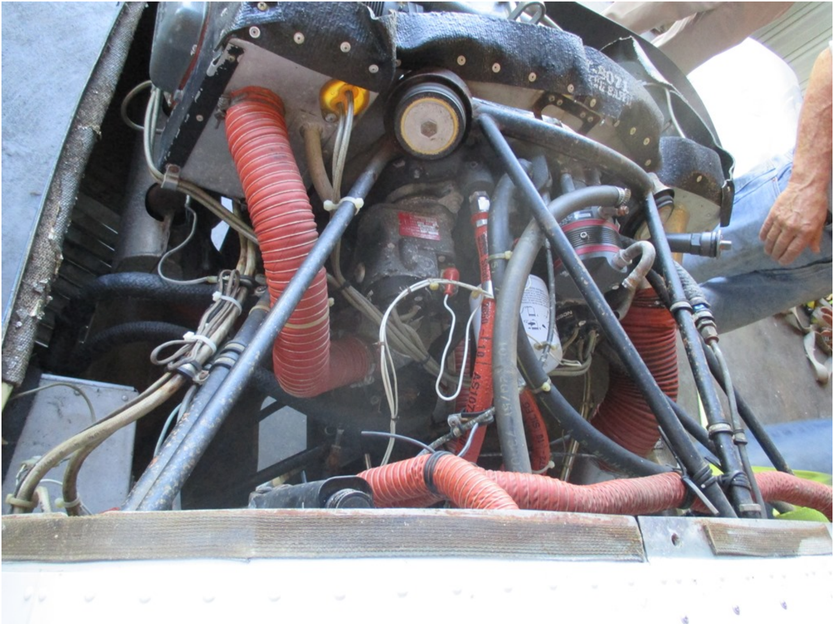
Photo 6 – Engine Hoses
