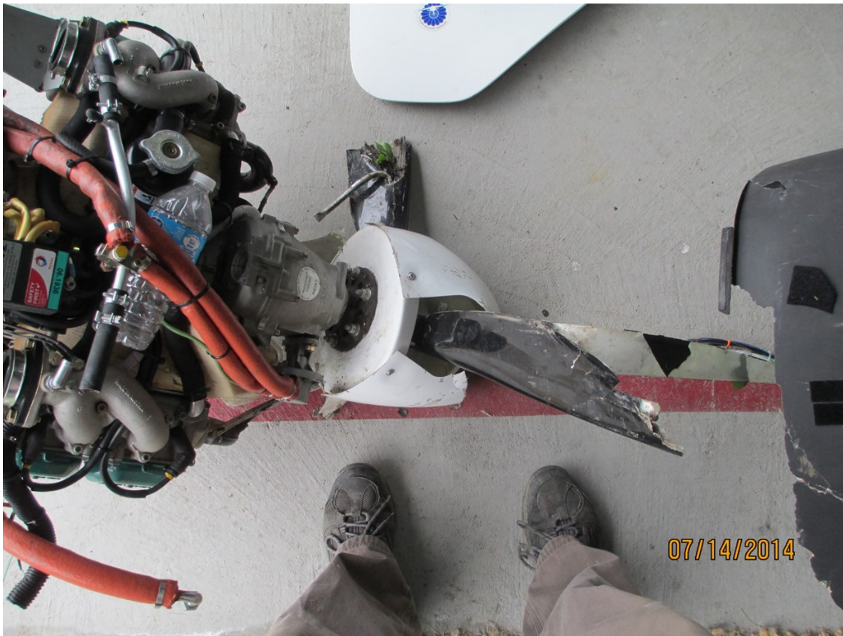
Photo 4 - Digital Photograph Provided By FAA. View of the Propeller and Portion of the Engine. Note the fractured Propeller Blades.
