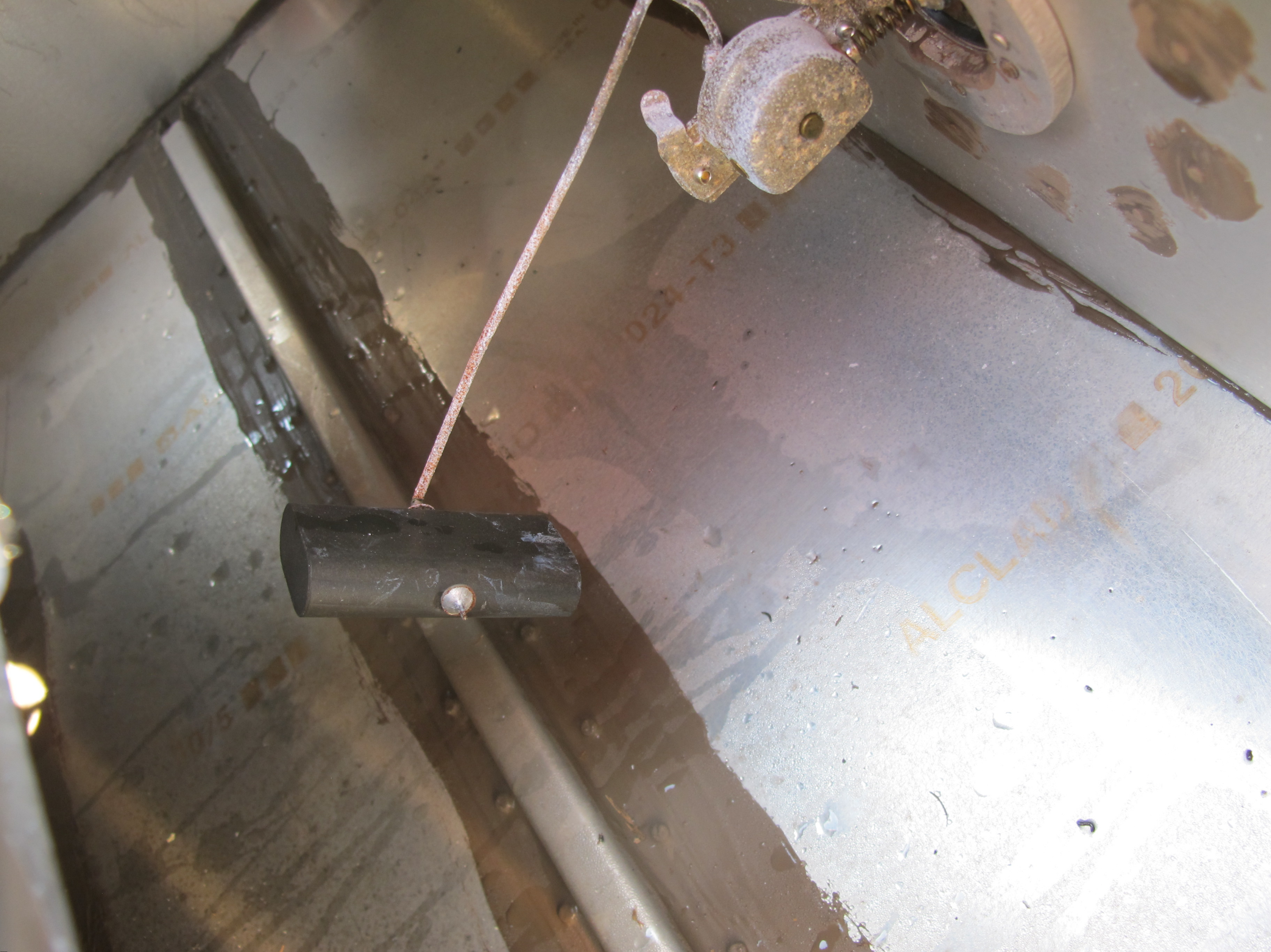
Photo 4 - Right Fuel Quantity Indicating Sensor (Photo Courtesy of Piper)
