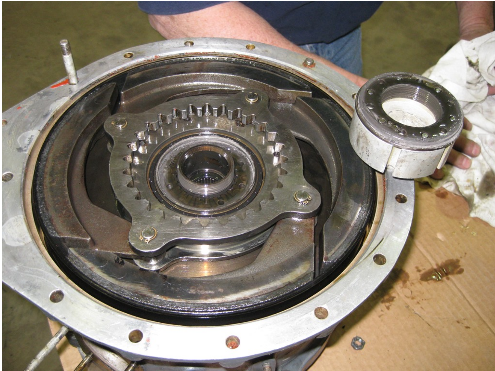
Photo 4 – Clutch Drum Housing – Courtesy of FAA
