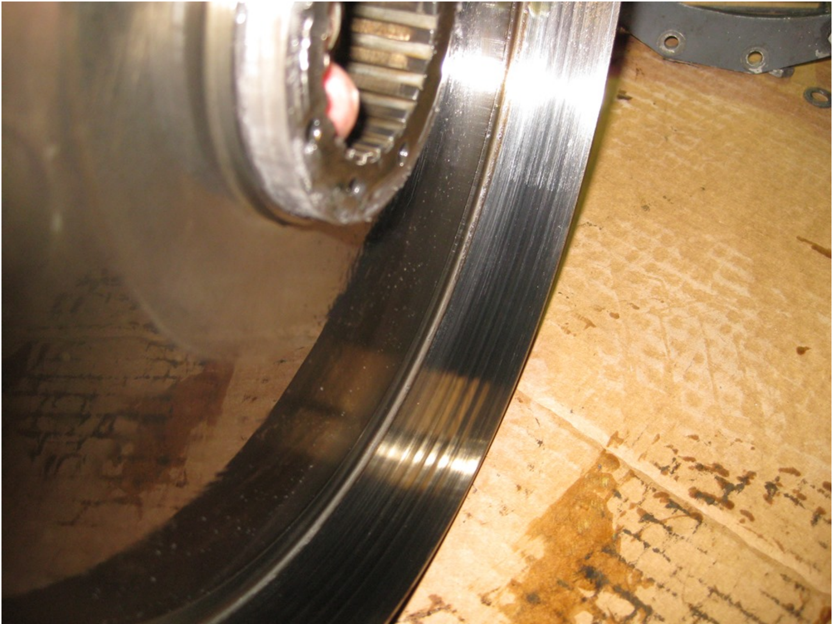
Photo 7 – Clutch Drum Wear – Courtesy of FAA
