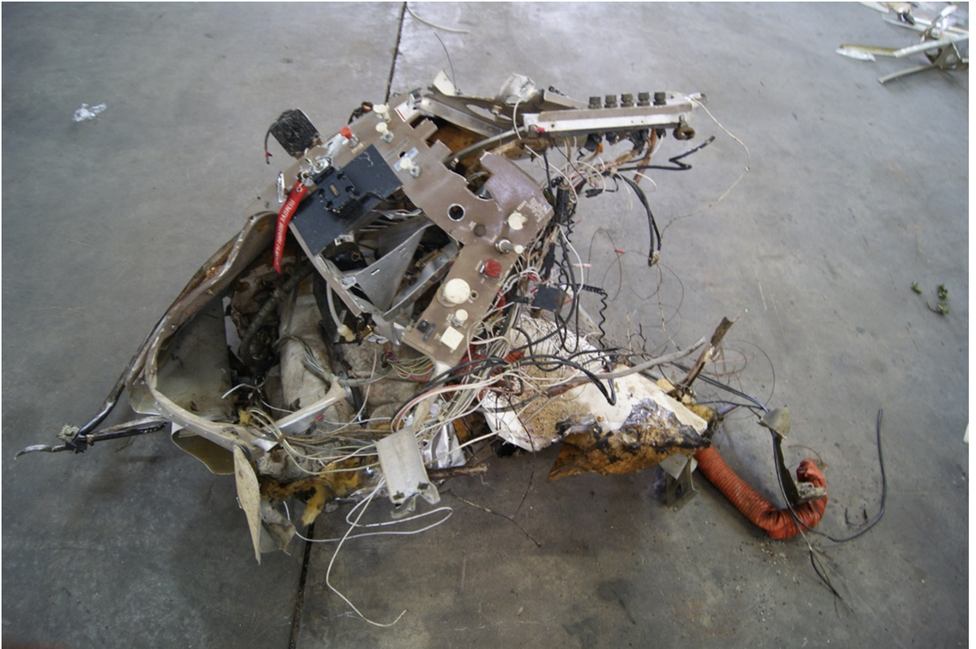
Photo 3 – Instrument Panel
