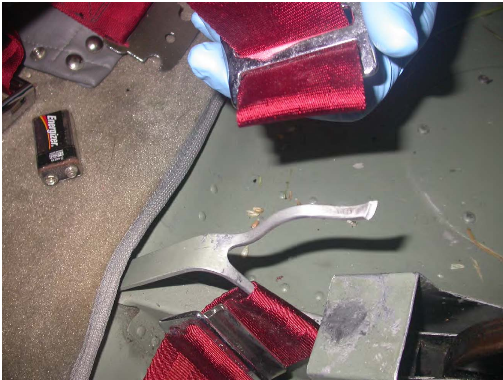
Photo 10 – Broken Center Safety Belt Bracket
