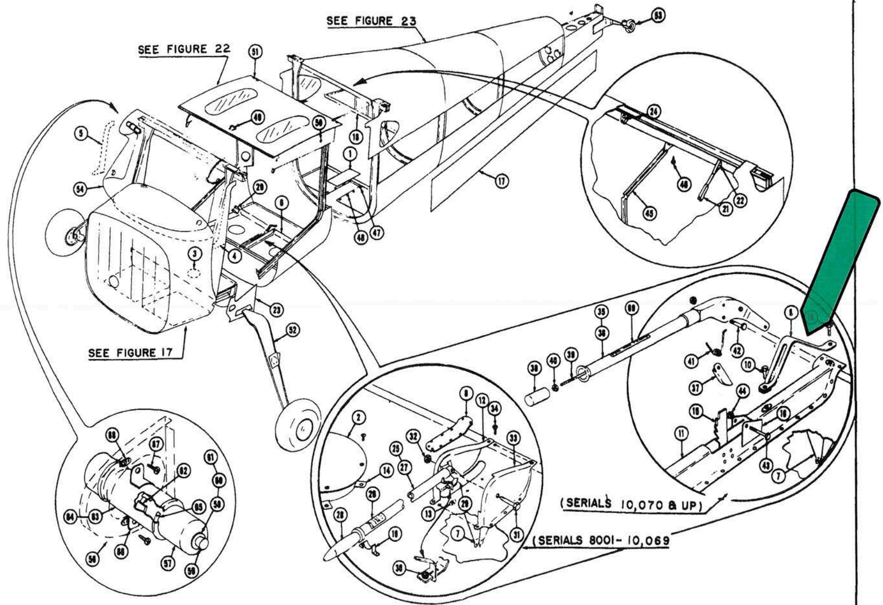
FIGURE 15-FUSELAGE ASSEMBLY COMPLETE
