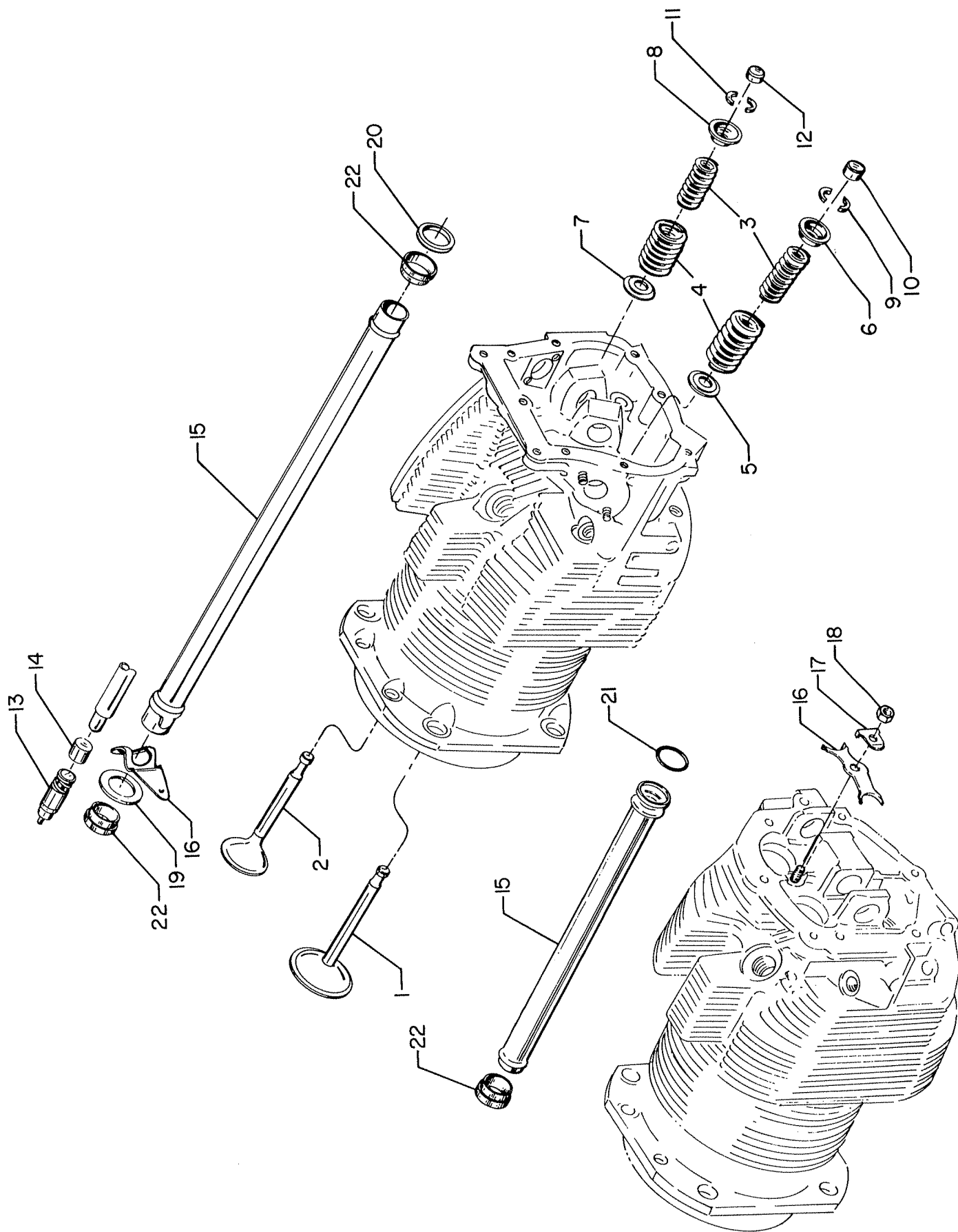
Figure 16 - Valve Assembly
