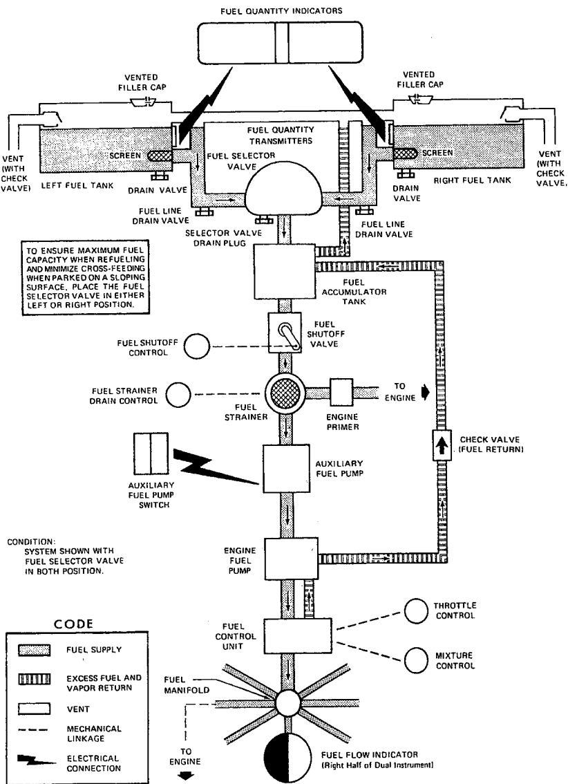
Figure 7-6. Fuel System
