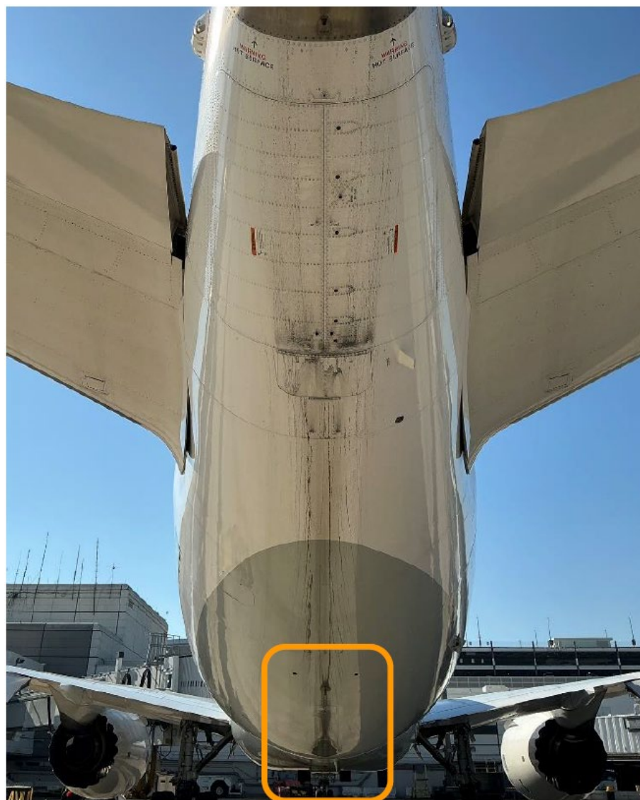
Photograph 1 - Damage to the lower fuselage. See photograph 2 for the area highlighted in the orange box. (Courtesy of ANA)
