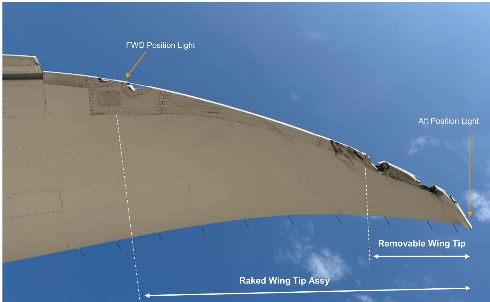
Damage Overview (bottom view)
