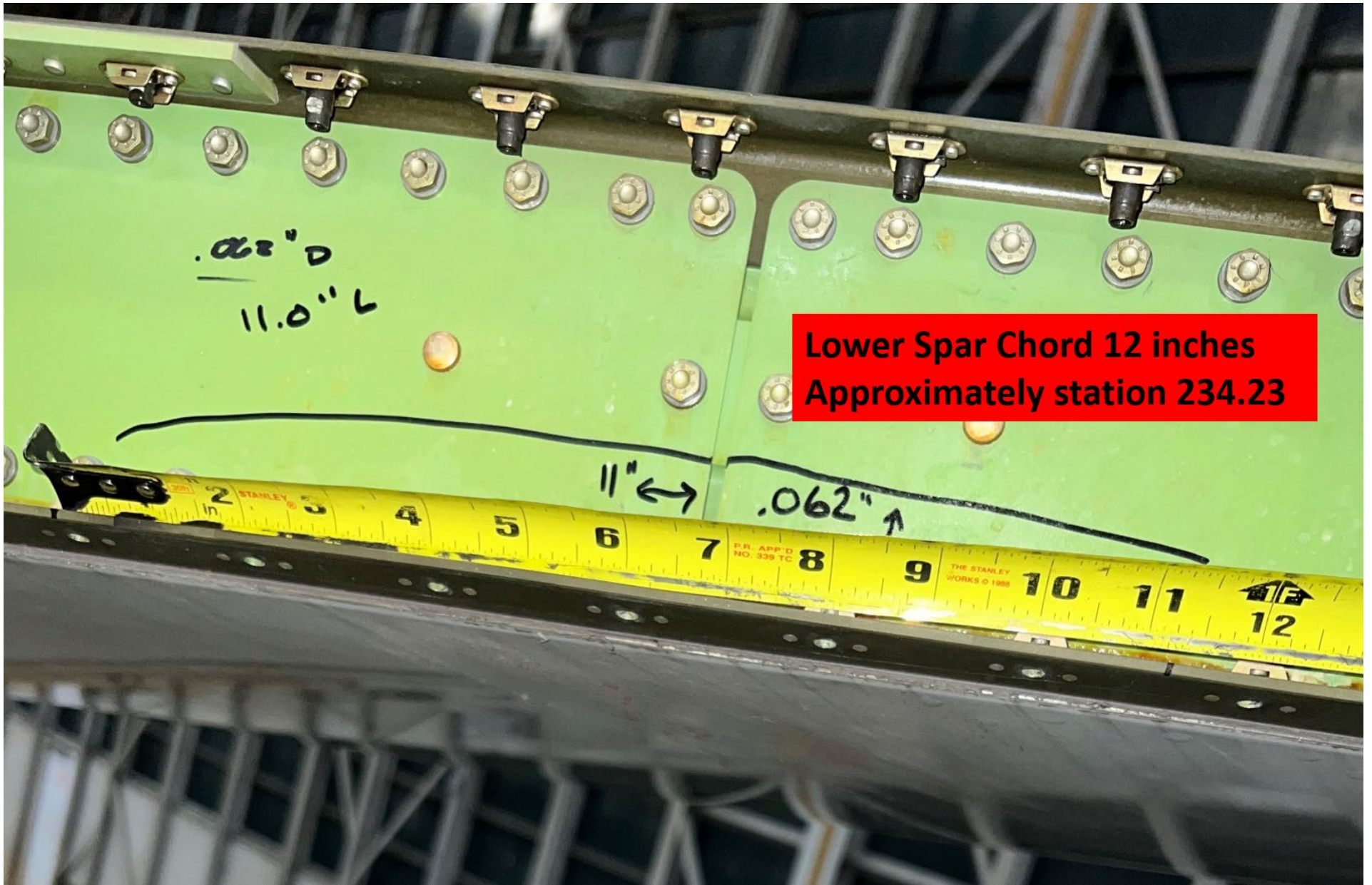
Left Horizontal Stabilizer Spar (courtesy SWA)
