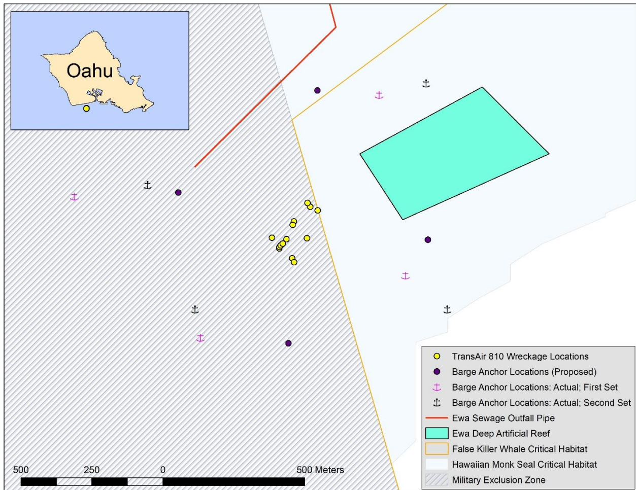
Figure 1. Barge proposed and actual anchor locations.
