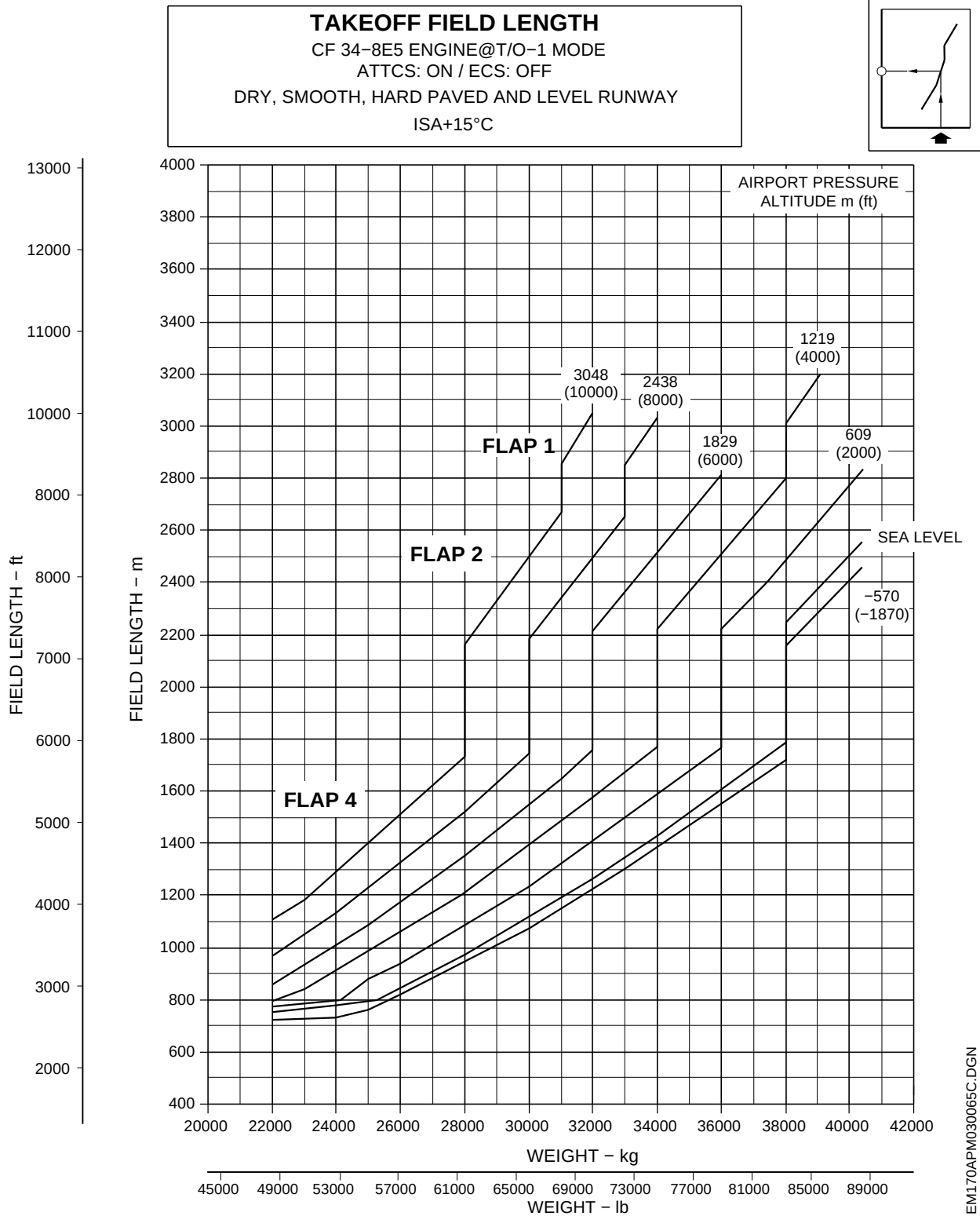
Takeoff Field Lengths - ISA + 15 °C Conditions Figure 3.6
