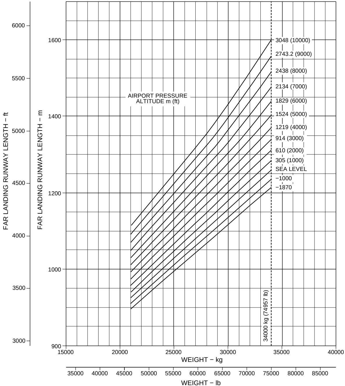
Landing Field Lengths - Flaps Full Figure 3.14
