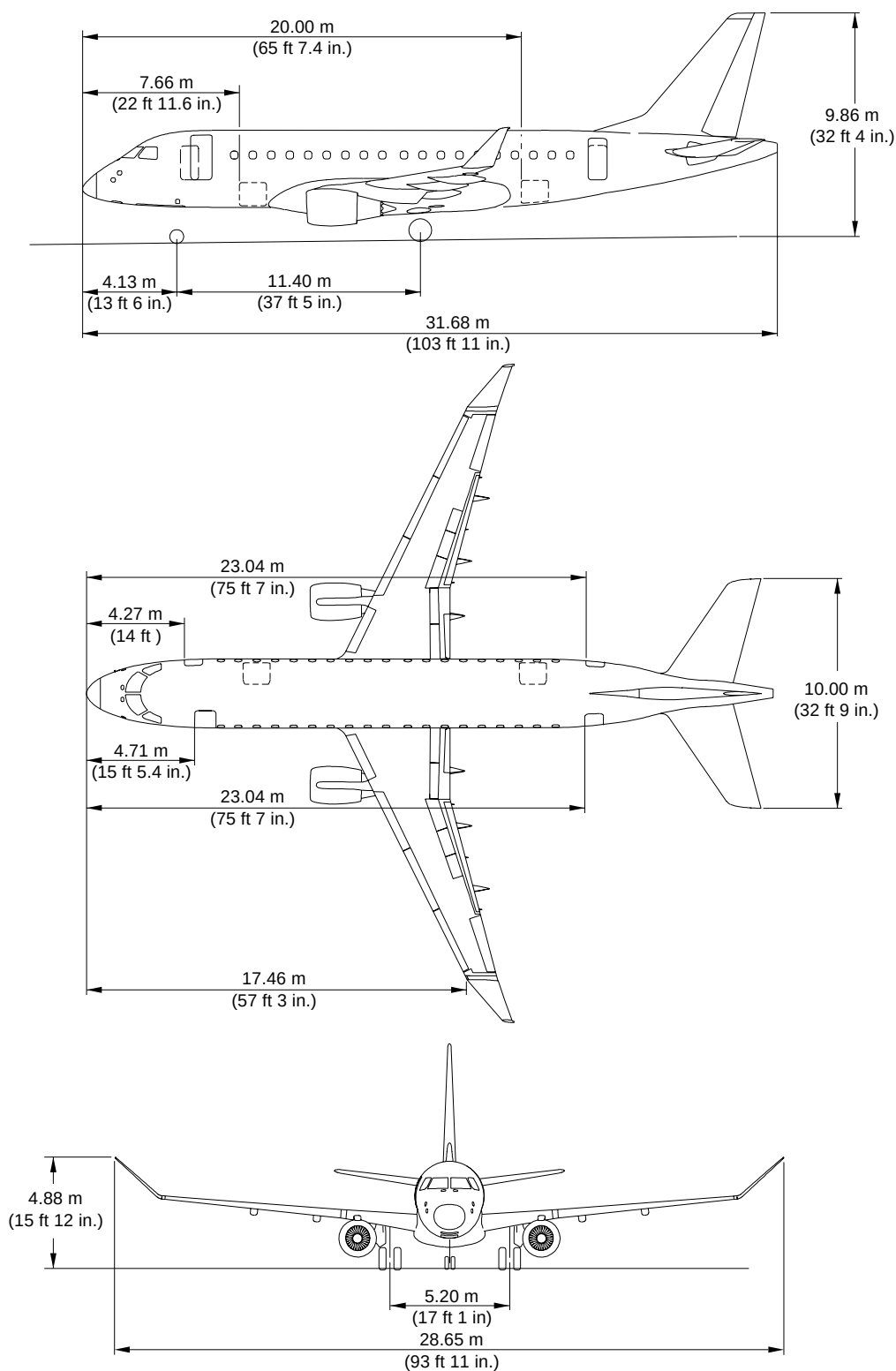
General Aircraft Dimensions Figure 2.2
