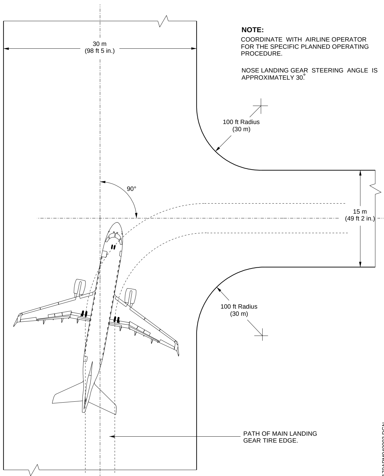
90° Turn - Runway to Taxiway Figure 4.8
