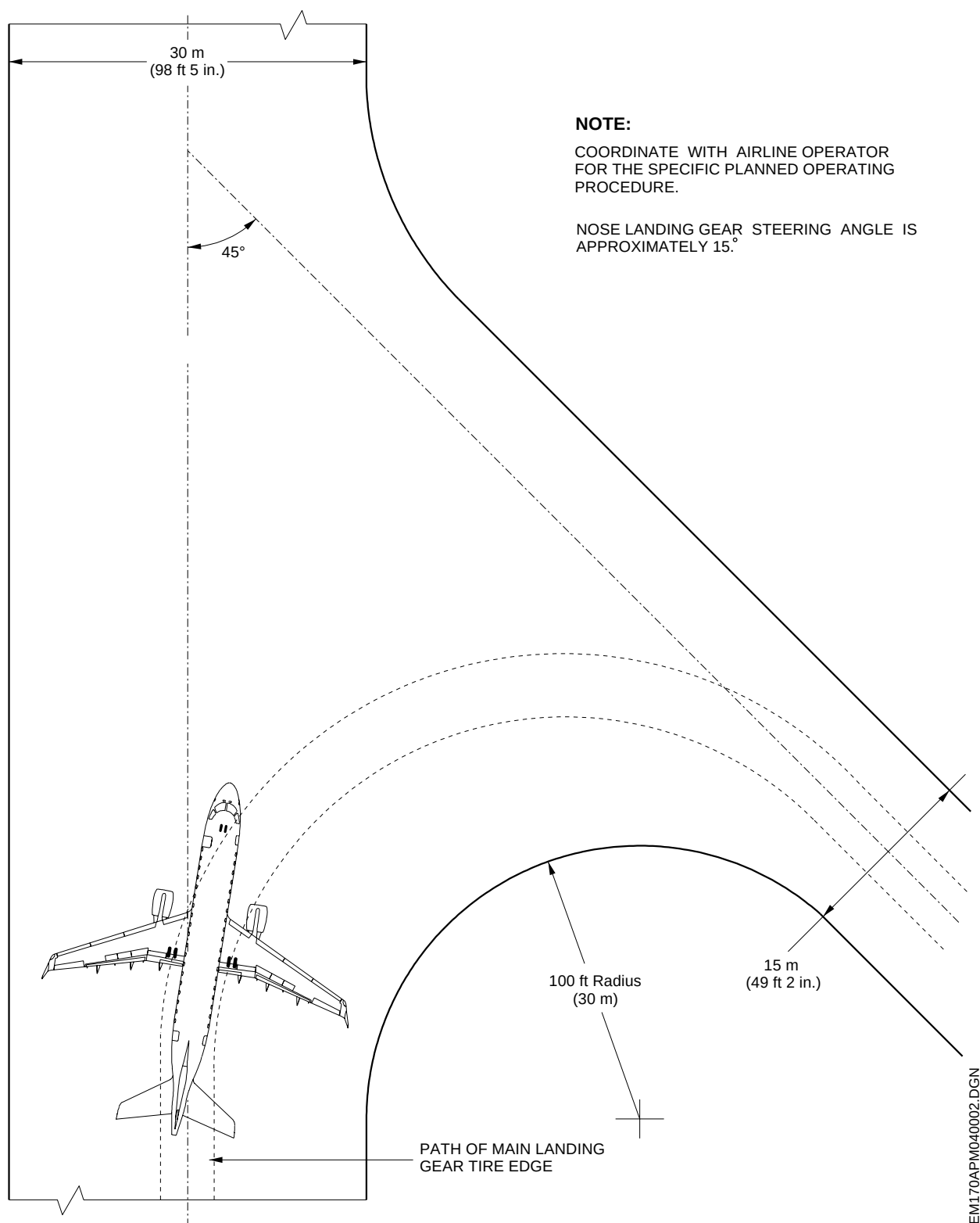
More than 90° Turn - Runway to Taxiway Figure 4.6
