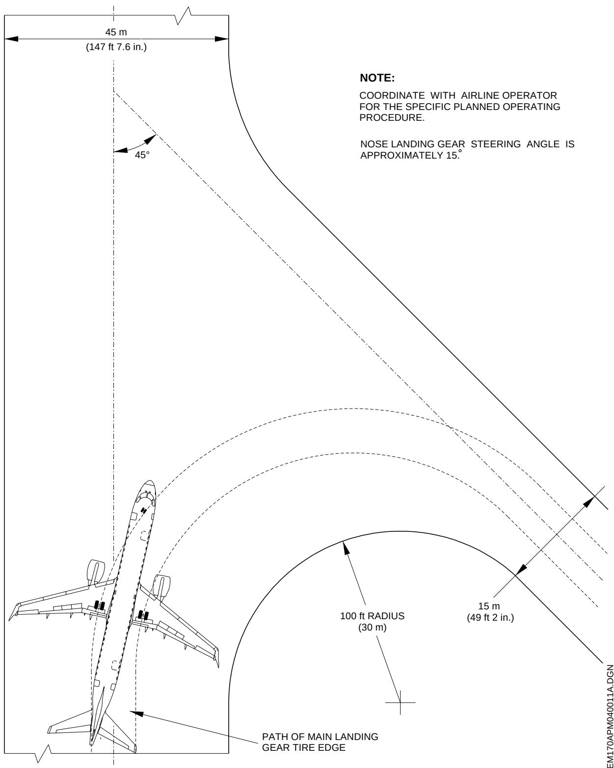
More than 90° Turn - Runway to Taxiway Figure 4.7
