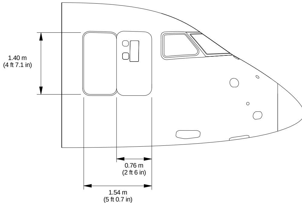
Passenger and Service Doors Dimensions Figure 2.3 Sheet 1
