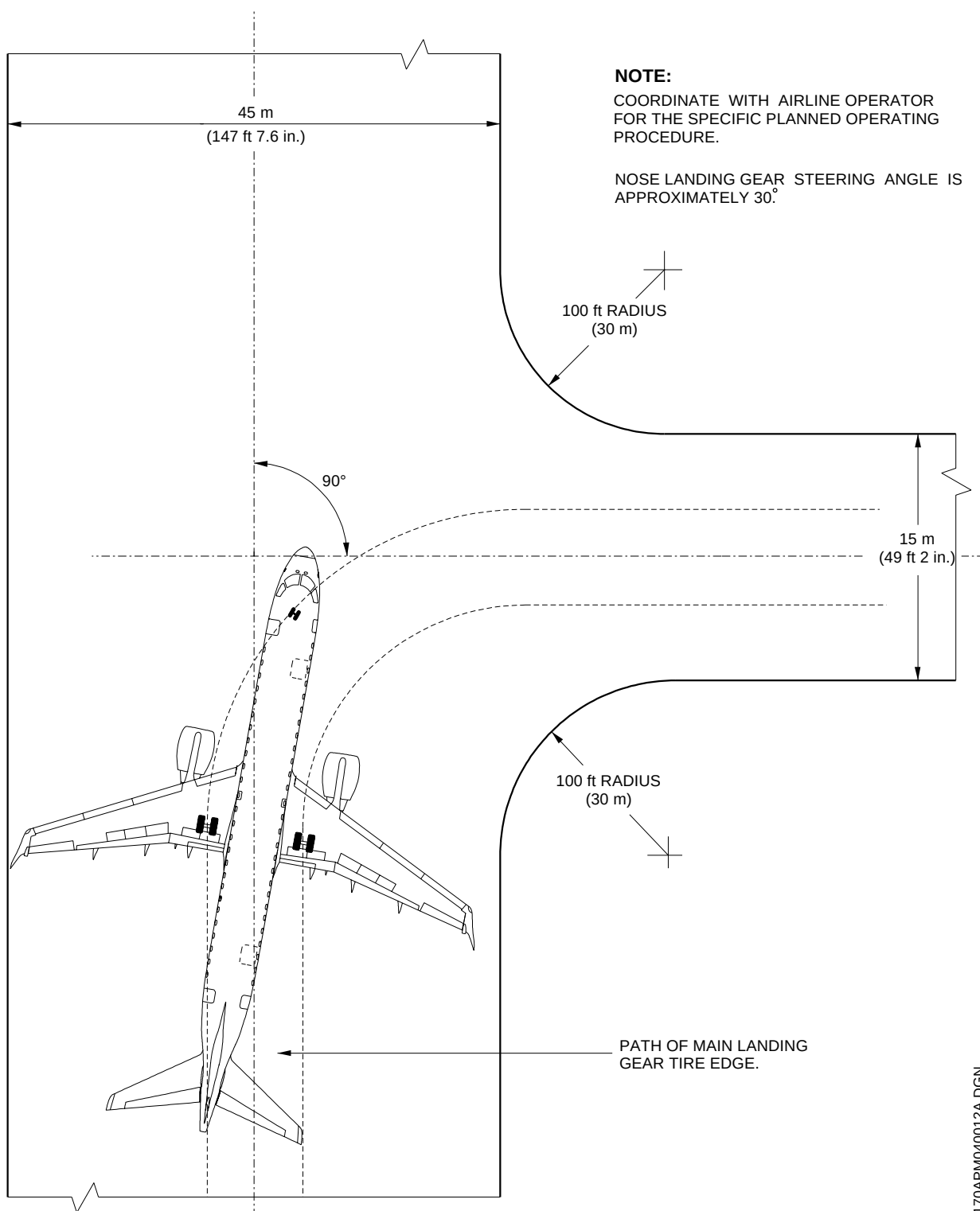
90° Turn - Runway to Taxiway Figure 4.9
