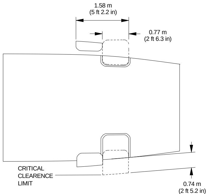
Passenger and Service Doors Dimensions Figure 2.3 Sheet 3
