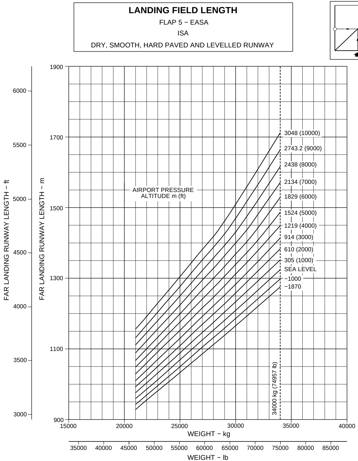
Landing Field Lengths - Flaps 5 Figure 3.15
