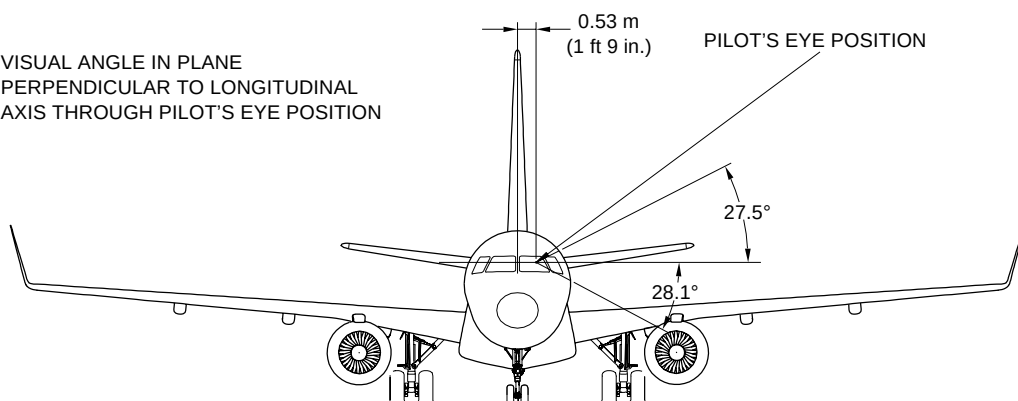
Visibility from Cockpit in Static Position Figure 4.5
