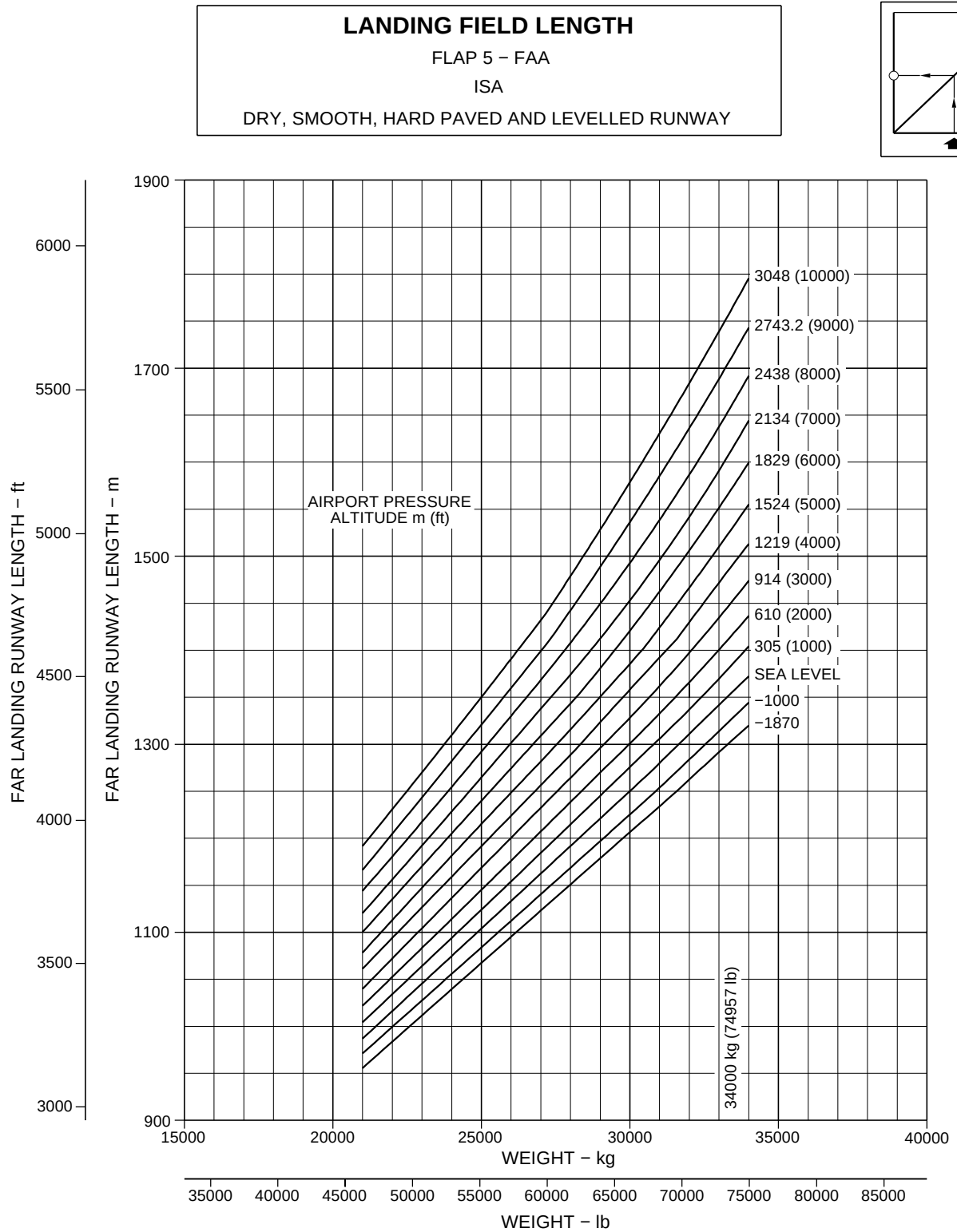
Landing Field Lengths - Flaps 5 Figure 3.13
