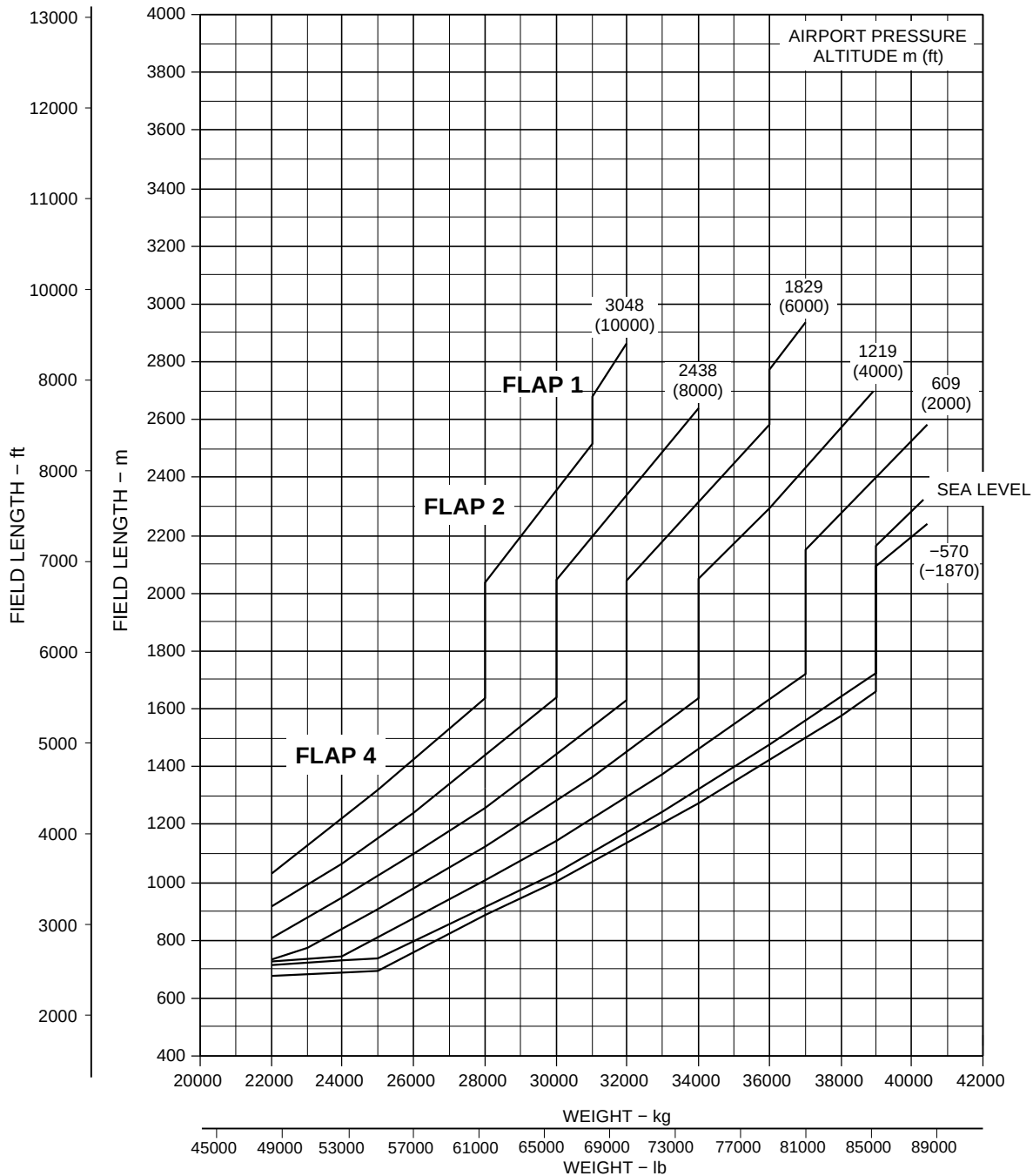
Takeoff Field Lengths - ISA Conditions Figure 3.9
