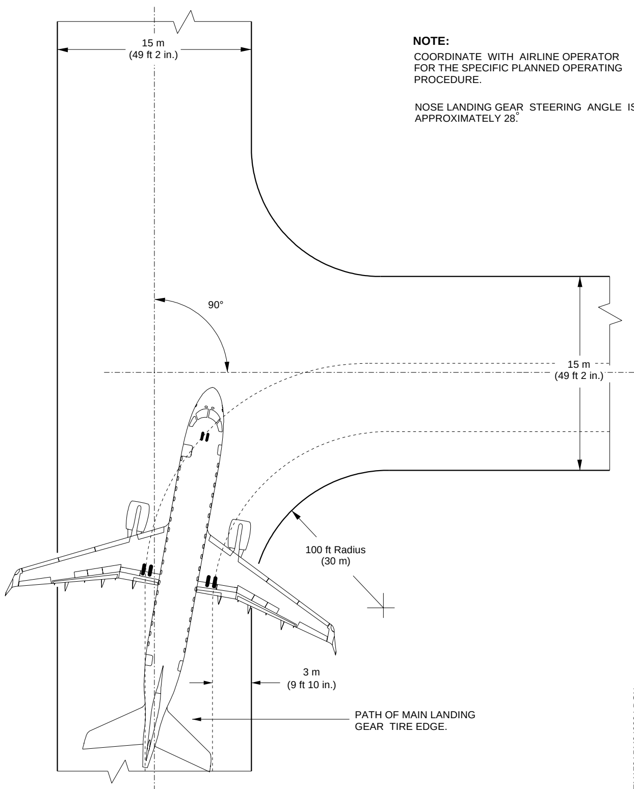
90° Turn - Taxiway to Taxiway Figure 4.10
