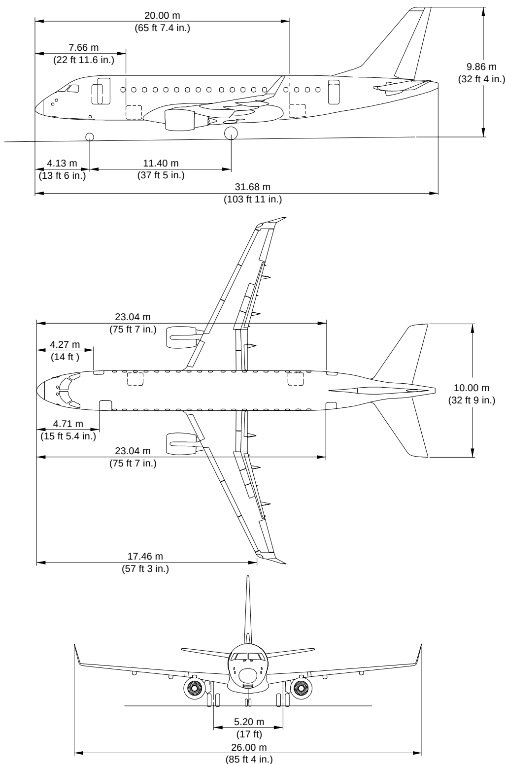
General Aircraft Dimensions Figure 2.1
