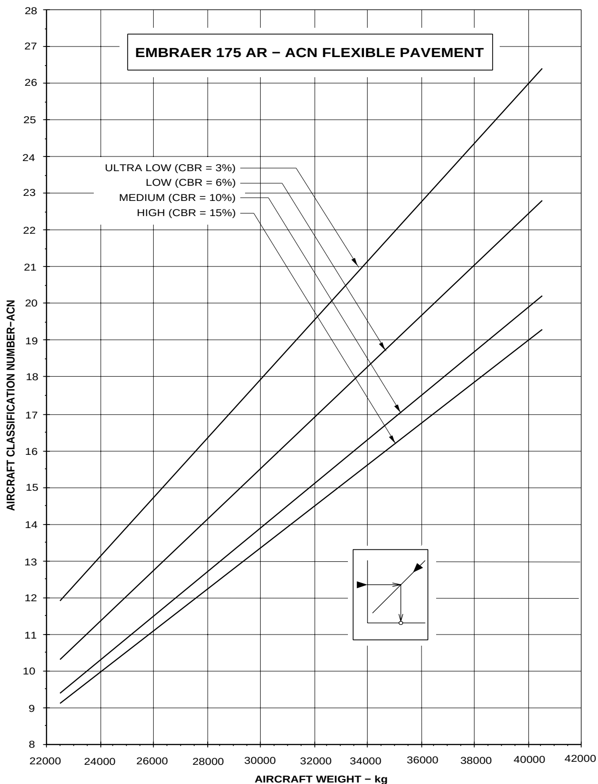
ACN For Flexible Pavement Figure 7.12
