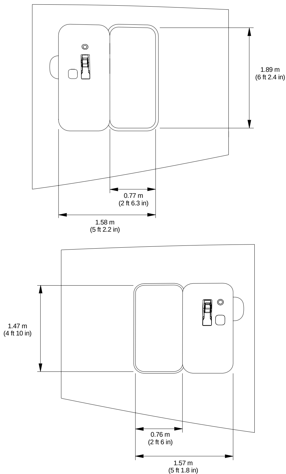
Passenger and Service Doors Dimensions Figure 2.3 Sheet 2
