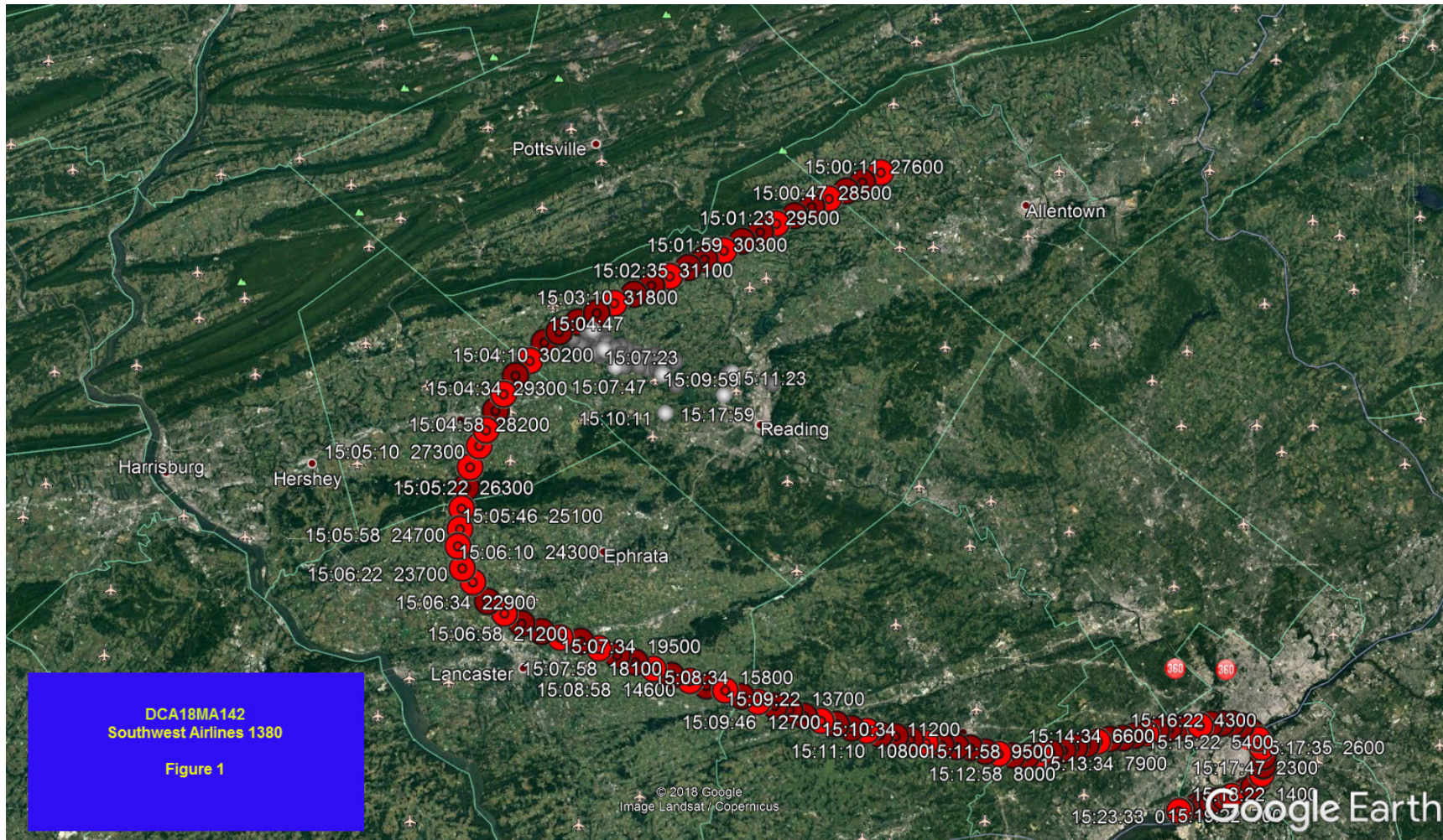
Figure 1 – FAA radar data showing the track of the accident aircraft. At 1103:3, the aircraft was at 32,500 feet.
