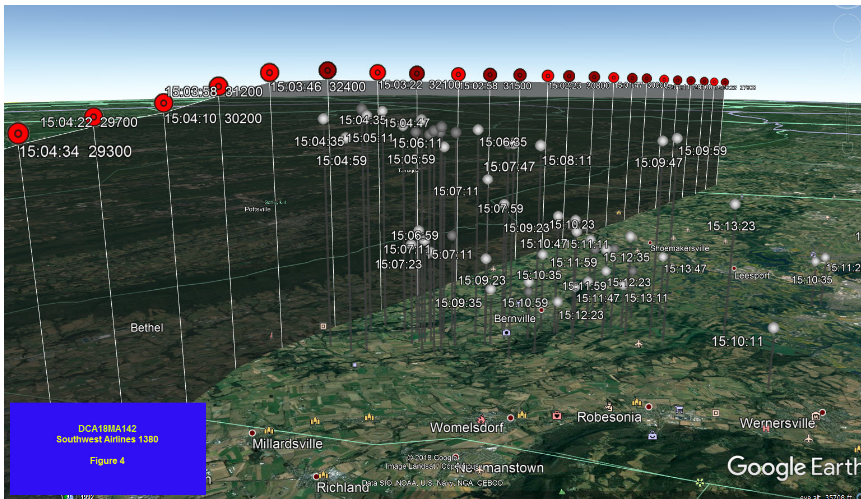
Figure 4 - Radar data showing the primary targets falling away from the flight track of the aircraft.
