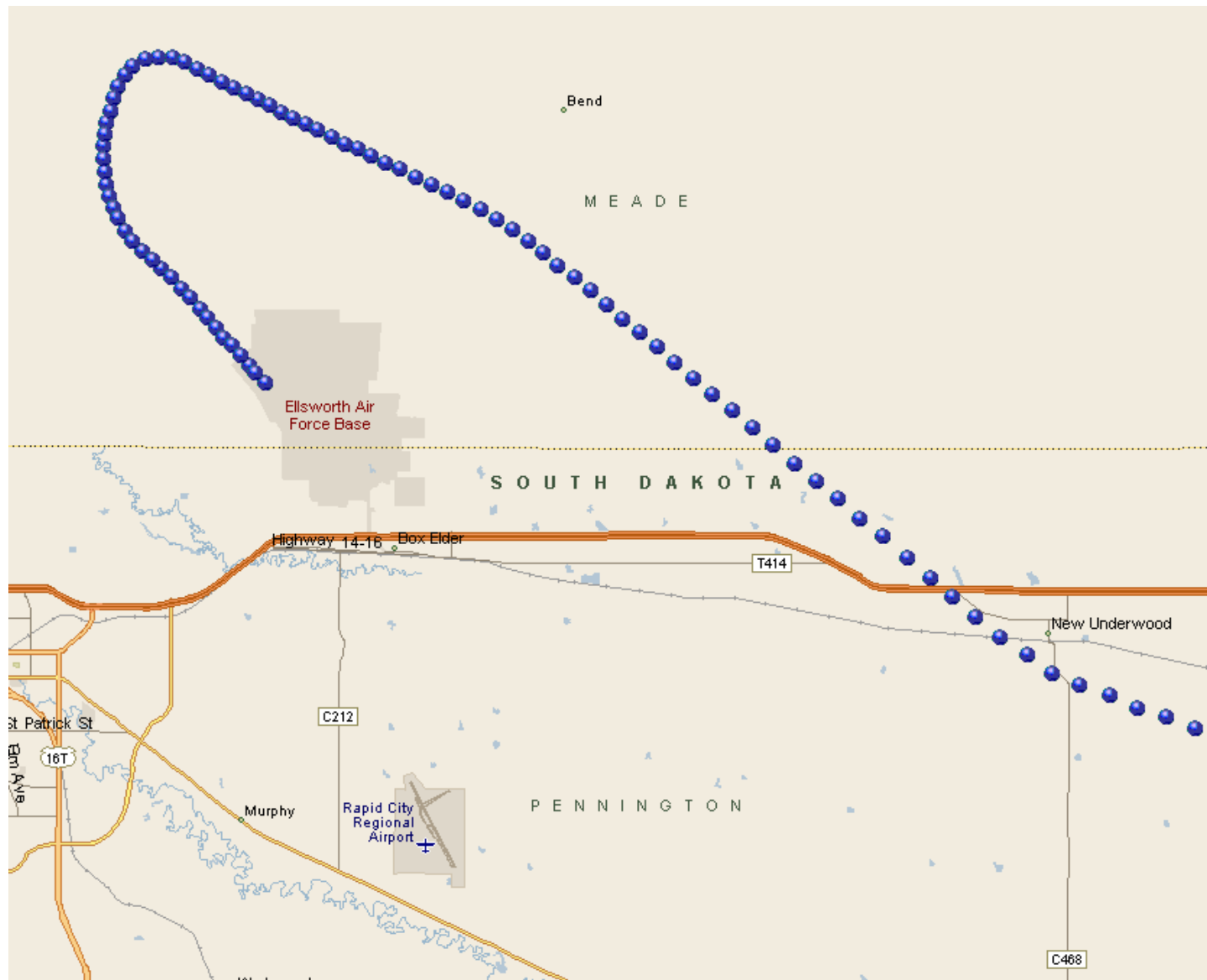
Figure 3 – DAL2845 track during vectors for the visual approach to RAP (located 6.45 nm SE of Ellsworth AFB).
