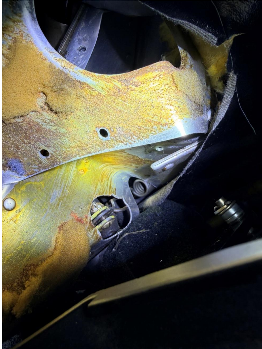
Photograph 3 - View of the substantial damage sustained to the lower fuselage near the cockpit (courtesy of the Federal Aviation Administration)
