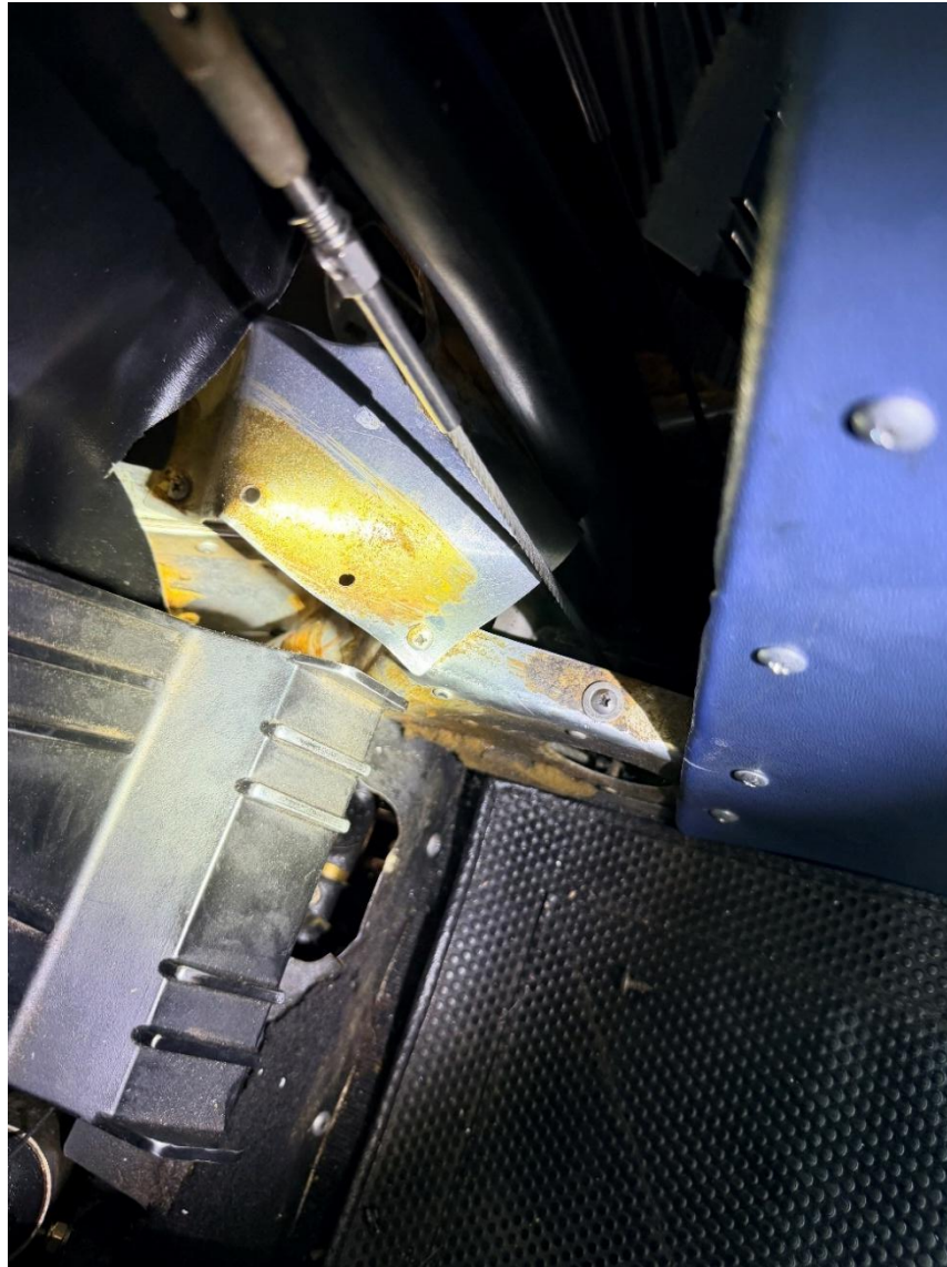
Photograph 2 - View of the substantial damage sustained to the lower fuselage near the cockpit (courtesy of the Federal Aviation Administration)
