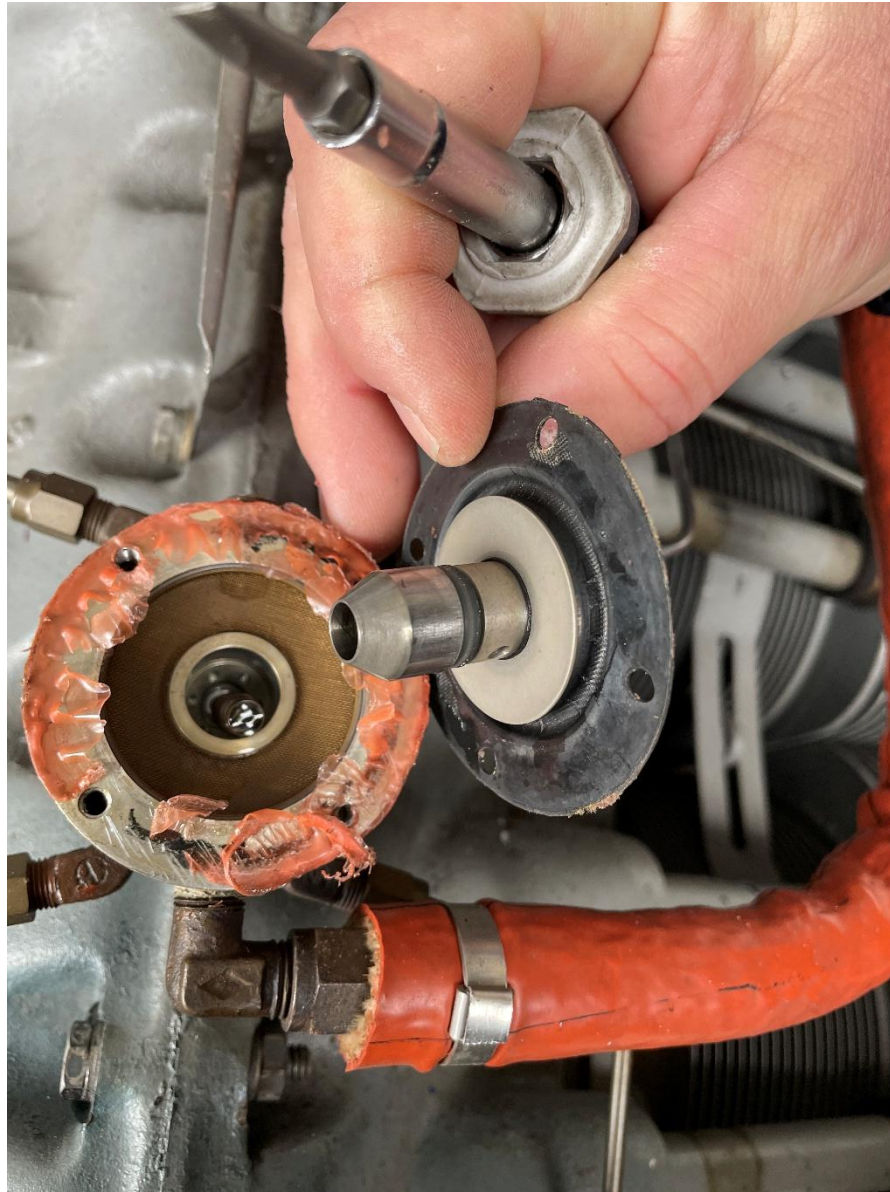
Photograph 8 - Fuel manifold top removed, no fuel noted (Courtesy of NTSB)
