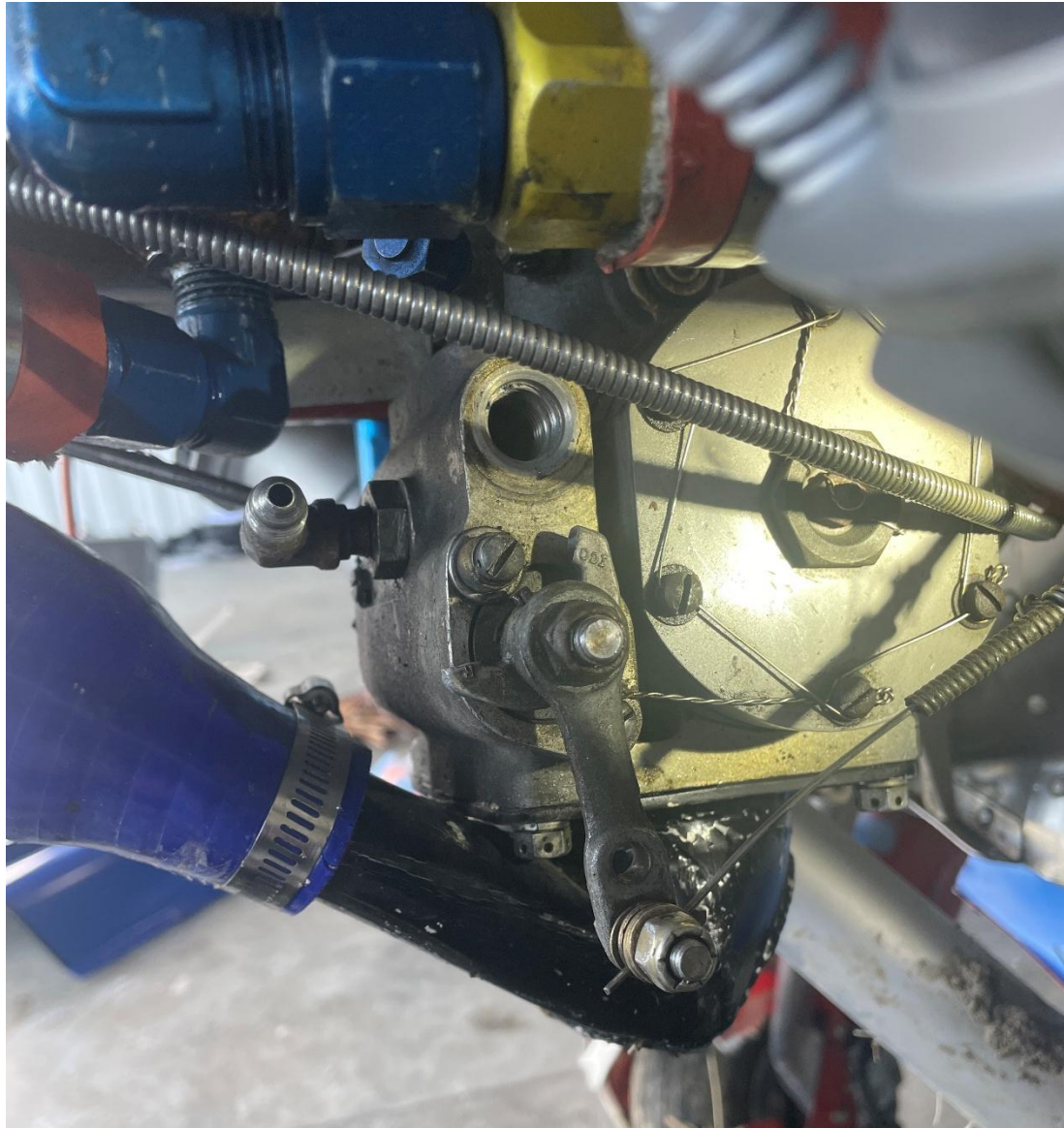
Photograph 6 - Position of mixture arm with fuel screen removed (Courtesy of NTSB)
