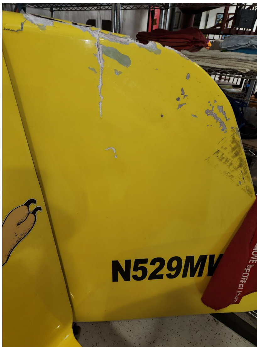
Photograph 2 - Accident Aircraft Rudder Damage (Courtesy of the Pilot)
