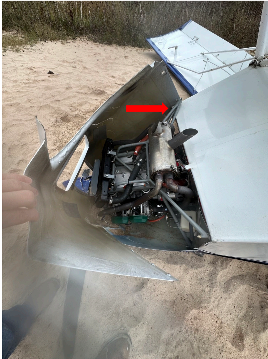
Photograph 3 - Broken engine mount (Courtesy of FAA)
