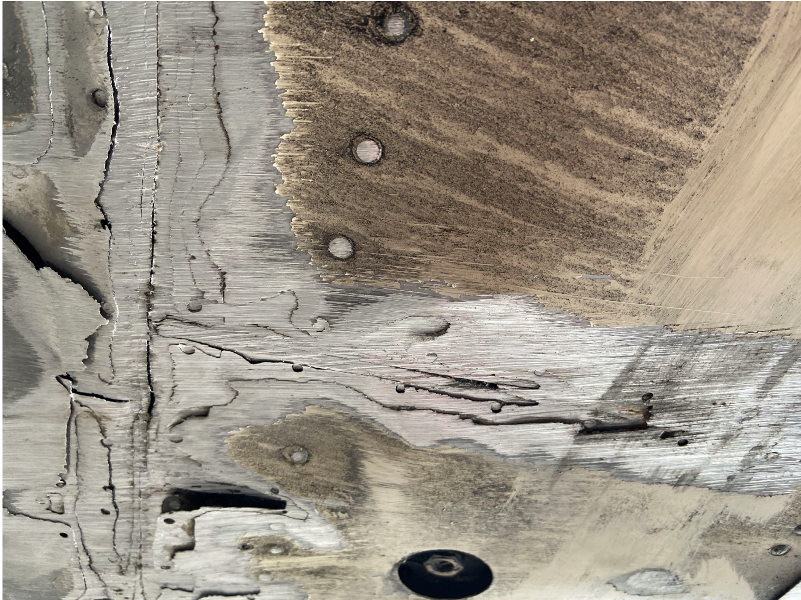
Photograph 2 - Fuselage damage (Courtesy of FAA)
