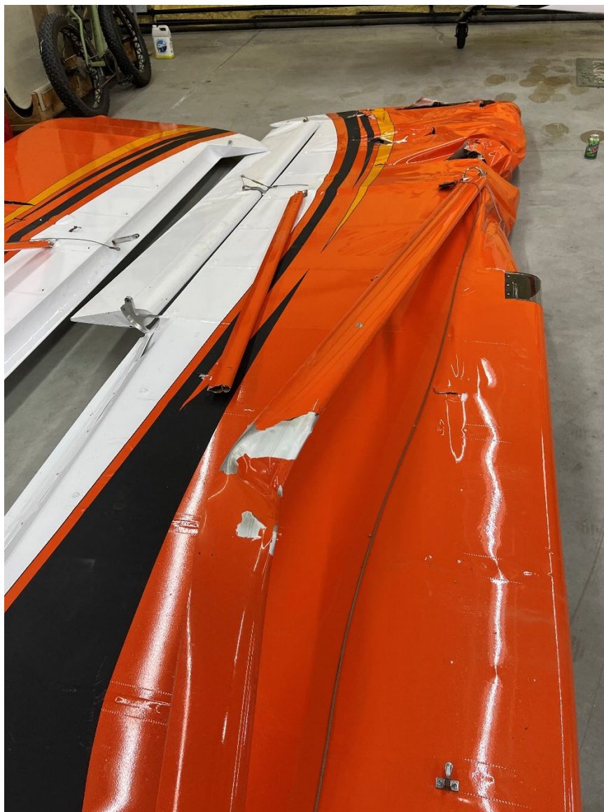
Photograph 5 - View of the right wing and the right wing strut (courtesy of the Federal Aviation Administration)
