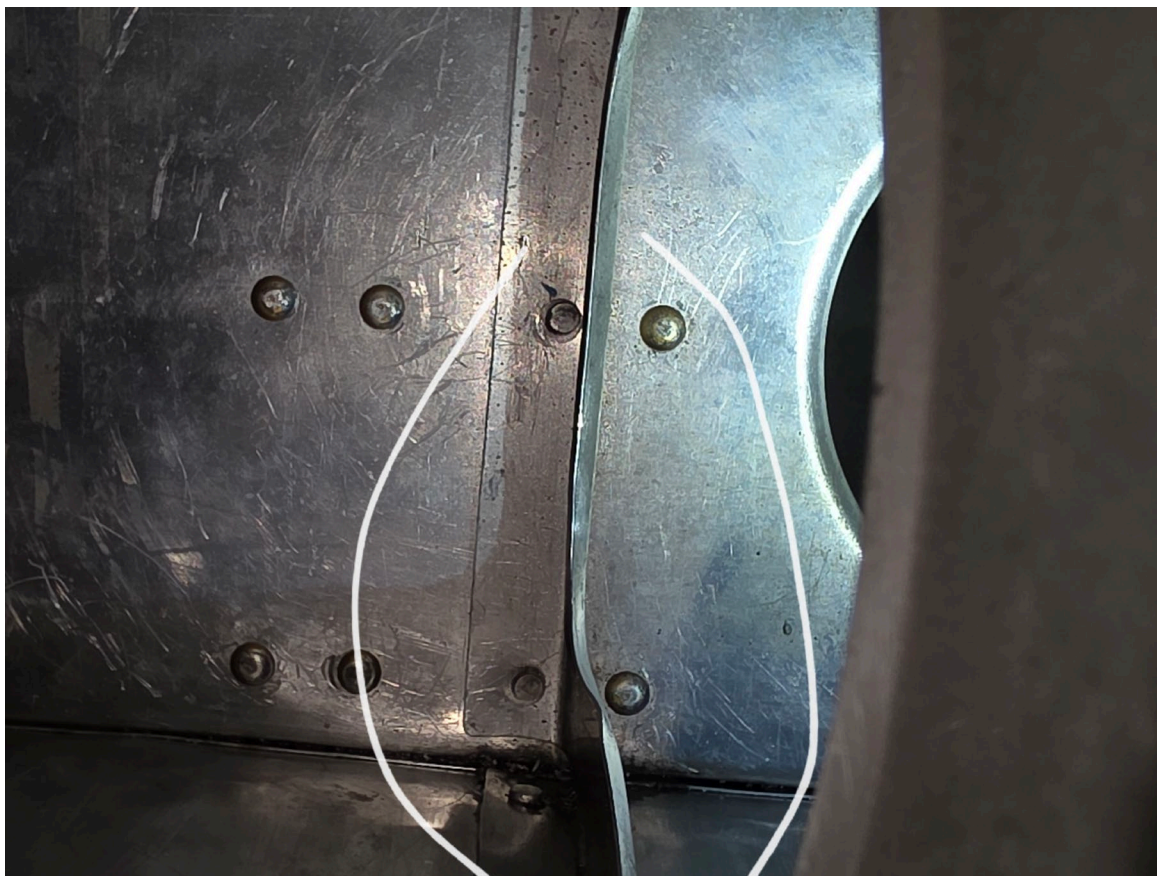
Photograph 2 - Rib Damage - Emphasis Added (Courtesy of USAFA Aero Club)
