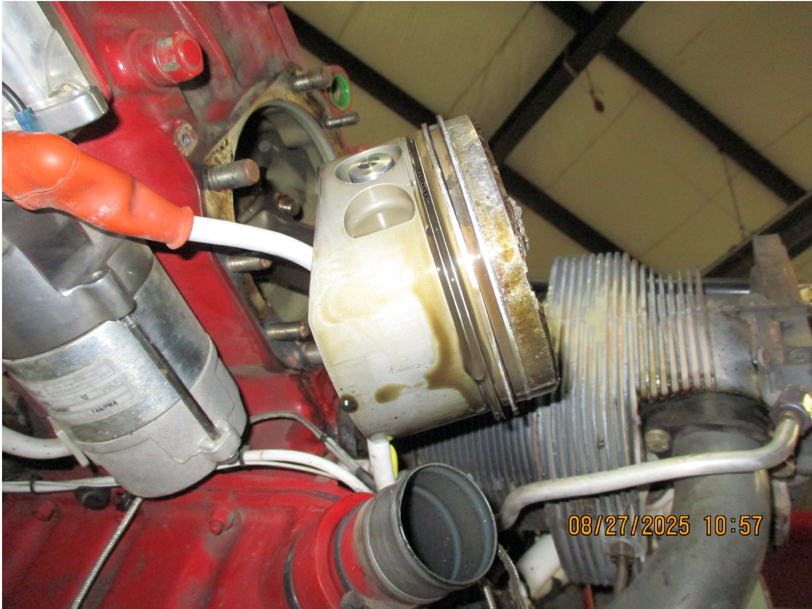
Photograph 5 - No. 2 piston (Courtesy of FAA)
