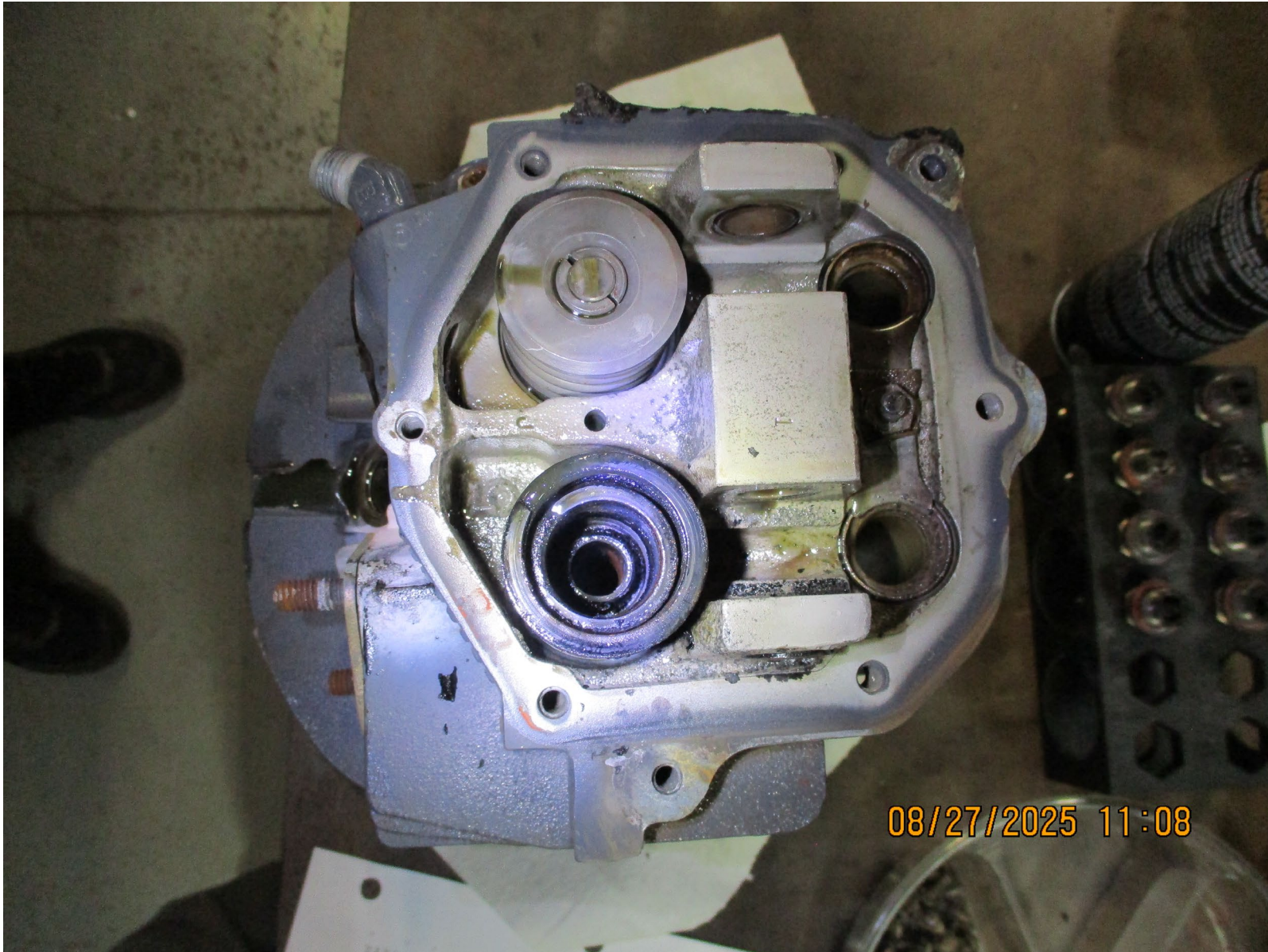
Photograph 7 - No. 2 cylinder (Courtesy of FAA)
