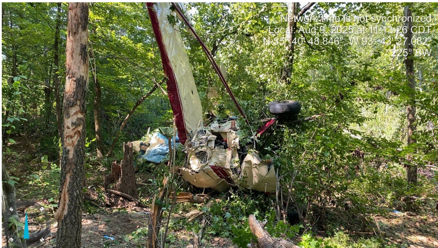
Photograph 2 - View of the front of the airplane at the accident site (courtesy of the Federal Aviation Administration)
