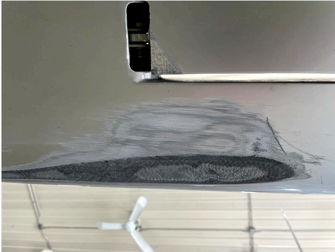
Photograph 2 -Damage to left wing (Courtesy of FAA)
